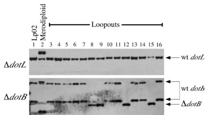
FIG. 3. dotL is an essential gene on bacteriological media. dotL and dotB merodiploids were constructed and recombinants selected as described in Fig. 2 were analyzed by Southern analysis (as described in Materials and Methods). The top panel shows a Southern blot of recombinants derived from a parental \Delta dotL/\Delta dotL merodiploid strain probed with a 700-bp SalI fragment of DNA adjacent to the dotL gene. Lane 1 is the wild-type strain Lp02; lane 2 is JV1003, a \Delta dotL/\dot{dotL} merodiploid; and lanes 3 to 16 are JV1003 plated on CYET plus 5% sucrose. All 14 strains that were selected for sucrose resistance in this fashion retained the wild-type version of dotL . In contrast, the bottom panel is a similar experiment in which sucrose resistant recombinants derived from a dotB / \Delta dotB merodiploid strain were probed with a dotB -region specific probe. Lane 1 is the wild-type strain Lp02; lane 2 is JV941, a dotB / \Delta dotB merodiploid; and lanes 3 to 16 are JV941 selected on CYET plus 5% sucrose. In this case, two distinct types of recombinants are observed, a finding consistent with either dotB or \Delta dotB , indicating that dotB is not an essential gene.
