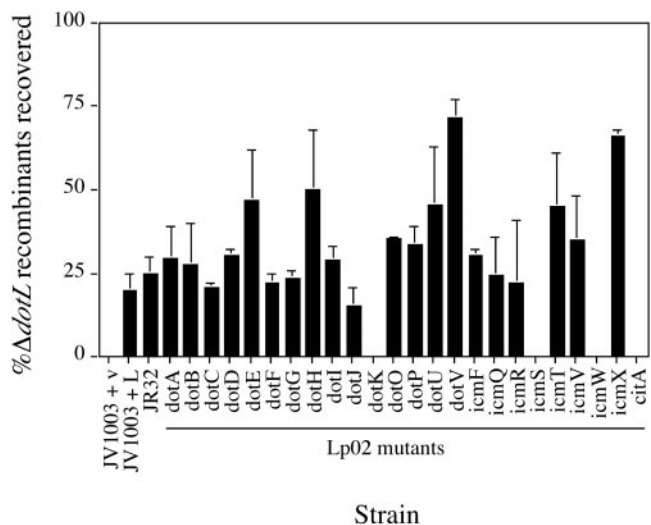
FIG. 6. Deletion of most dot/icm genes can suppress the lethality caused by deletion of dotL . A dotL / \Delta dotL ::Cm r merodiploid was constructed in a variety of different dot/icm backgrounds. Sucrose-resistant recombinants were selected and then screened for the \Delta dotL allele by resistance to chloramphenicol. \Delta dotL recombinants could not be obtained from the dotL / \Delta dotL ::Cm r merodiploid strain JV1003. The presence of a wild-type copy of dotL on a low-copy vector allowed the isolation of \Delta dotL recombinants (JV1003 plus dotL ). Inactivation of 20 of 23 dot/icm genes suppressed the loss of dotL . In addition, deletion of citA / tpxA , a housekeeping gene found near the dot/icm genes, did not allow loss of dotL (42). In contrast, dotL is not essential in a related L. pneumophila strain, JR32. The data shown reflects the average number of \Delta dotL recombinants recovered from scoring 50 events from four independent experiments.
