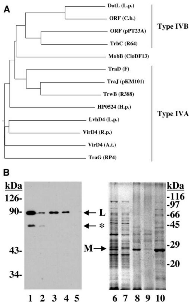
FIG. 1. (Top) DotL shows sequence similarity to members of the T4CP family. DotL has extensive similarity to a number of putative type IVB secretion system ATPases, including an uncharacterized ORF in Coxiella burnetii [ORF (C.b.)], the TrbC protein of the IncI plasmid R64 [TrbC (R64)], and a TrbC orthologue on the pPT23A plasmid of Pseudomonas syringae strains [ORF (pPT23A)]. DotL has similarity to plasmid T4CPs (MobB, TraD, TraJ, TrwB, and TraG from the plasmids CloDF13, F, pKM101, R388, and RP4, respectively) and to T4CPs from adapted conjugation systems found in pathogens (HP0524 from Helicobacter pylori , VirD4 from the Ti plasmid of Agrobacterium tumefaciens , and a VirD4 orthologue from Rickettsia prowazekii ). Most strains of L. pneumophila contain at least one additional T4CP, LvhD4, which is part of a second type IV secretion system (51). The dendrogram was generated by using CLUSTAL W alignment. (Bottom) The DotL protein is localized to the inner membrane of L. pneumophila . Extracts of wild-type L. pneumophila were separated into cytoplasmic and membrane fractions by high-speed centrifugation. The membrane fractions were then further separated into inner membrane versus outer membrane fractions by extraction with the detergent Triton X-100. Duplicate samples were run on two 7.5% acrylamide gels; the first gel was transferred to a polyvinylidene difluoride membrane and probed with anti-DotL serum (lanes 1 to 5), whereas the second gel was stained with Coomassie blue for total protein (lanes 6 to 10). Lanes 1 and 6 are total cell lysates, lanes 2 and 7 are soluble cytoplasmic fractions, lanes 3 and 8 are total membrane, lanes 4 and 9 are Triton X-100 soluble (inner membrane), and lanes 5 and 10 are Triton X-100 insoluble (outer membrane). All samples were loaded proportionally except for lanes 8, 9, and 10, which were overloaded in order to detect the protein profile (lane 8 is 3-fold, lane 9 is
