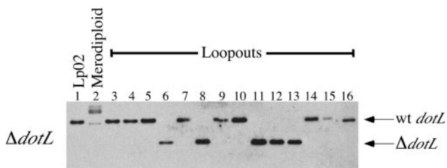
FIG. 5. The dotL gene can be deleted in a strain lacking dotA . Southern blot analysis of \Delta dotL recombinants in a \Delta dotA background. A 700-bp S all fragment from pJB1001 encoding DNA flanking dotL on the chromosome was used as a probe to determine the status of dotL in these strains. Lane 1 is the wild-type strain Lp02; lane 2 is JV1005, a \Delta dotL / dotL merodiploid in a dotA mutant background; and lanes 3 to 16 are JV1005 resolved on CYET plus 5% sucrose.
