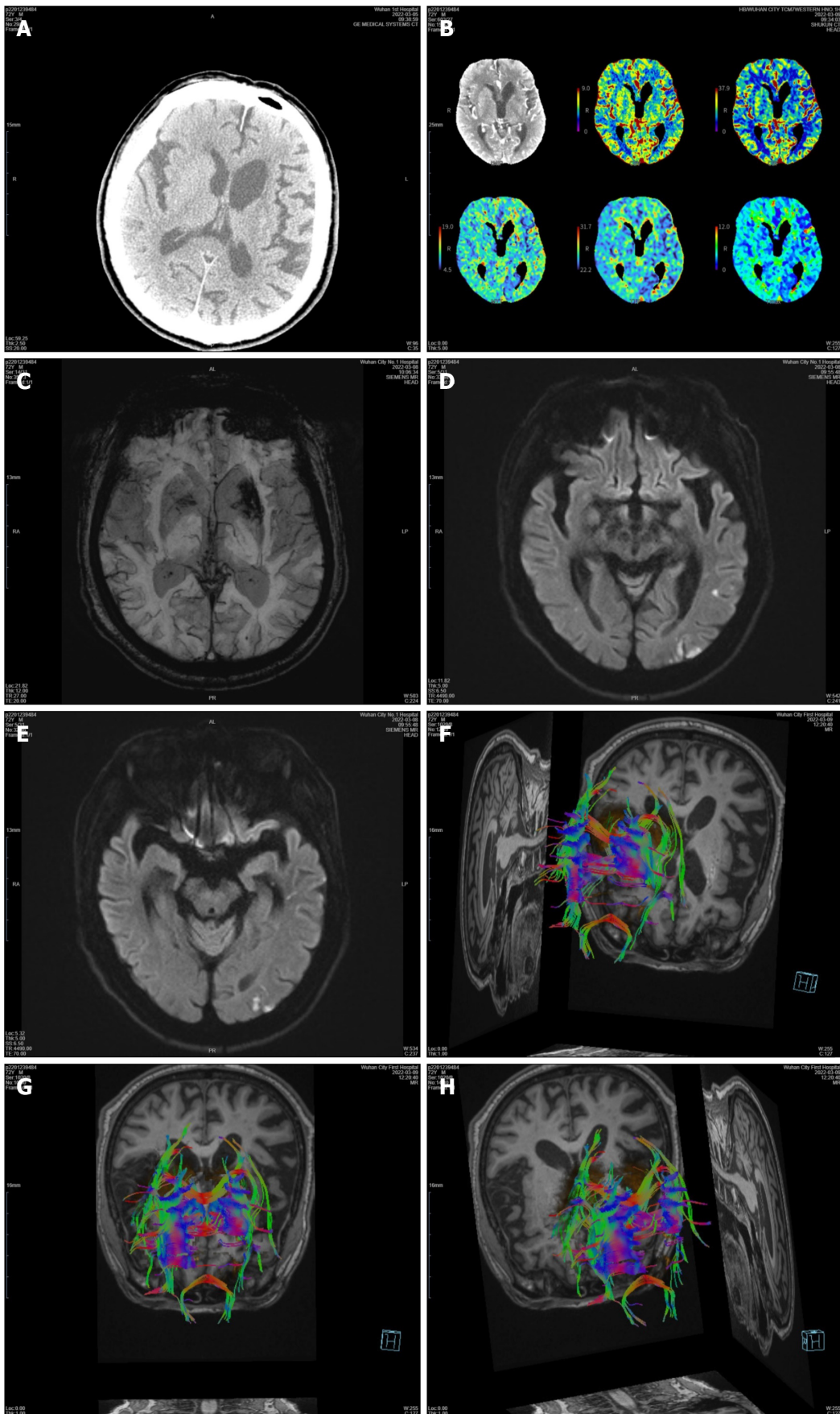
Figure 3 Neuroimaging of patient 2. A: Computed tomography of the head showed no hyperdensity; B: Computed tomography perfusion showed no abnormalities, with normal perfusion of the basal ganglia; C: Susceptibility weighted imaging showed low signal intensity in the left basal ganglia; D and E: Diffusion-
