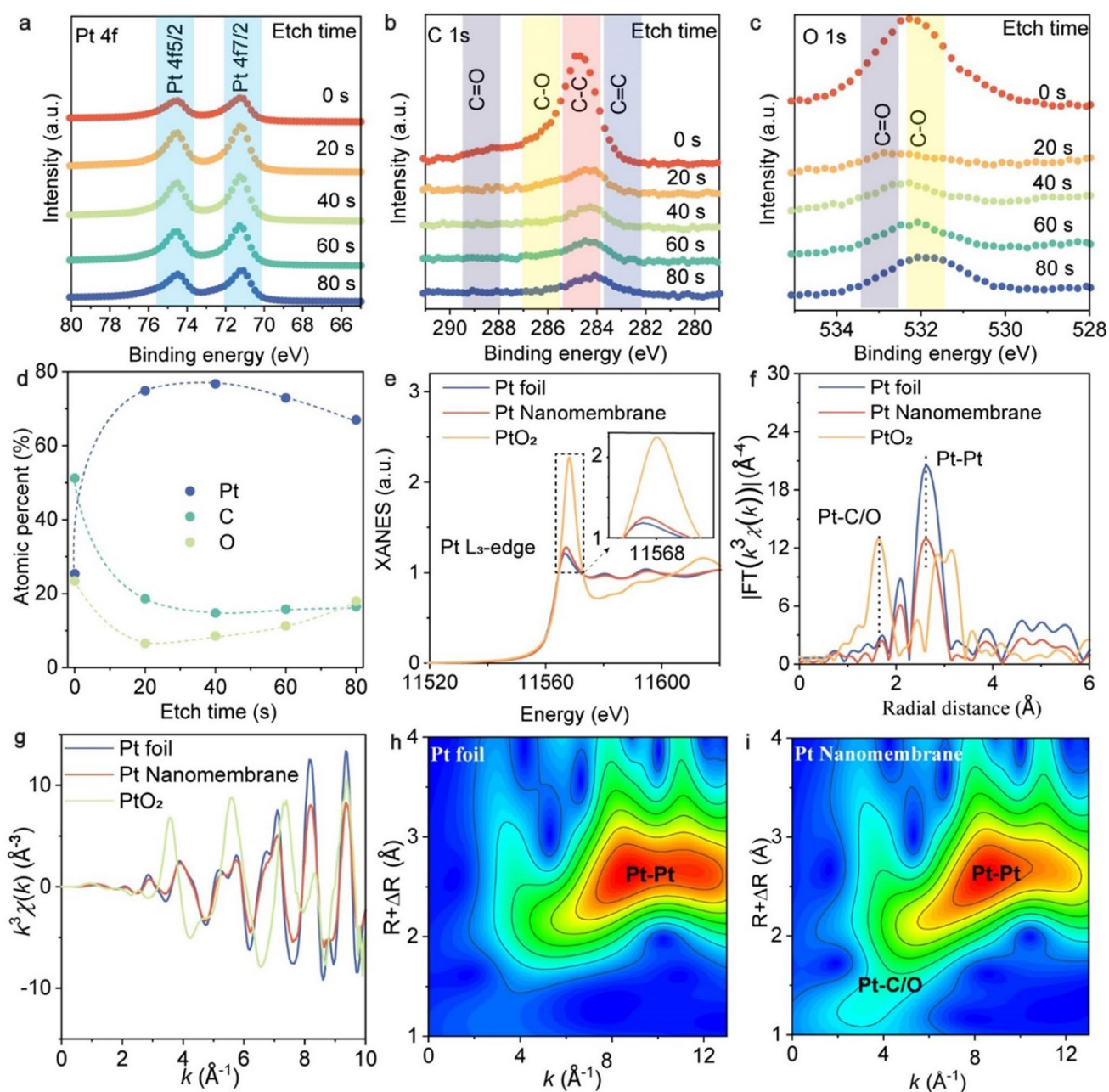
Fig. 2 Chemical bonding and atomic packing analyses of our 19 nm Pt nanomembranes. a–c X-ray photoelectron spectroscopy (XPS) depth profile analysis of Pt nanomembrane. Narrow-scan XPS spectra for a Pt 4f, b C 1s, and c O 1s as a function of etching time. d Relative atomic concentration of Pt, C, and O with etching time, as obtained from the quantitative analysis of the XPS. e X-ray absorption near edge structure (XANES) at Pt L 3 edge. f FT-EXAFS region for the local structure of Pt. g EXAFS \chi(k) signals in k -space. h and i show the wavelet transform for the k_3 -weighted EXAFS Pt K -edge signal of Pt foil and Pt nanomembrane, respectively
