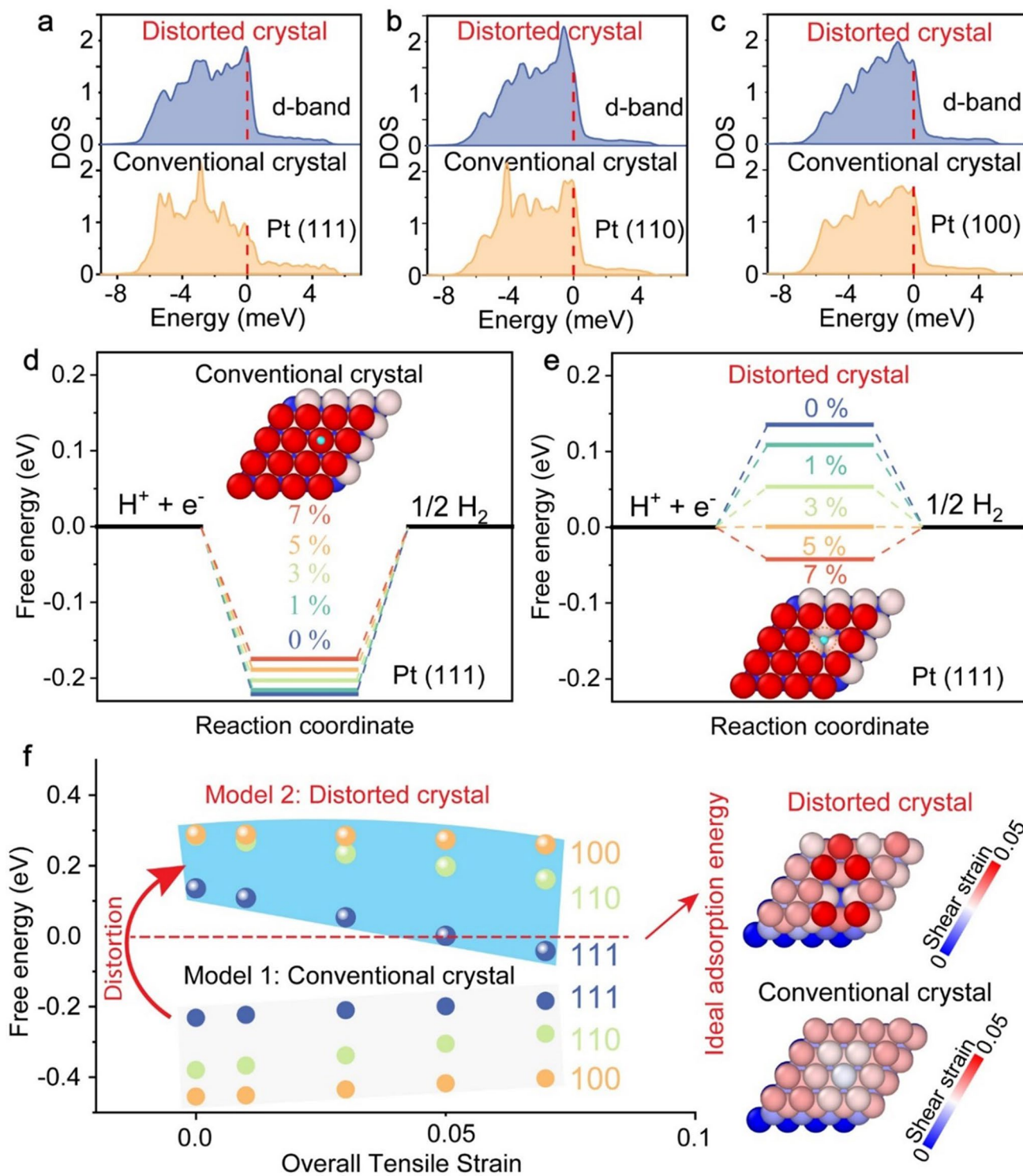
Fig. 4 The atomic and electronic origin of excellent HER activity on our Pt nanomembrane made up of severely distorted nanocrystals. a–c Projected density of states (DOS) on pristine Pt and distorted Pt surface at crystal orientation (111), (110), and (100), respectively, the dot line indicates Fermi level. d Adsorption free energy versus the reaction coordinate of HER for a conventional crystal with the uniform tensile strain ranging from 0 to 7%. e Adsorption free energy versus the reaction coordinate of HER for a distorted crystal with the heterogeneous tensile strain of 0–7%. f Comparison of free energy vs strain between a conventional and a distorted crystal with the orientation of (111), (110), and (100), insets are the strain mappings of a distorted crystal and conventional crystal at the orientation (111)
