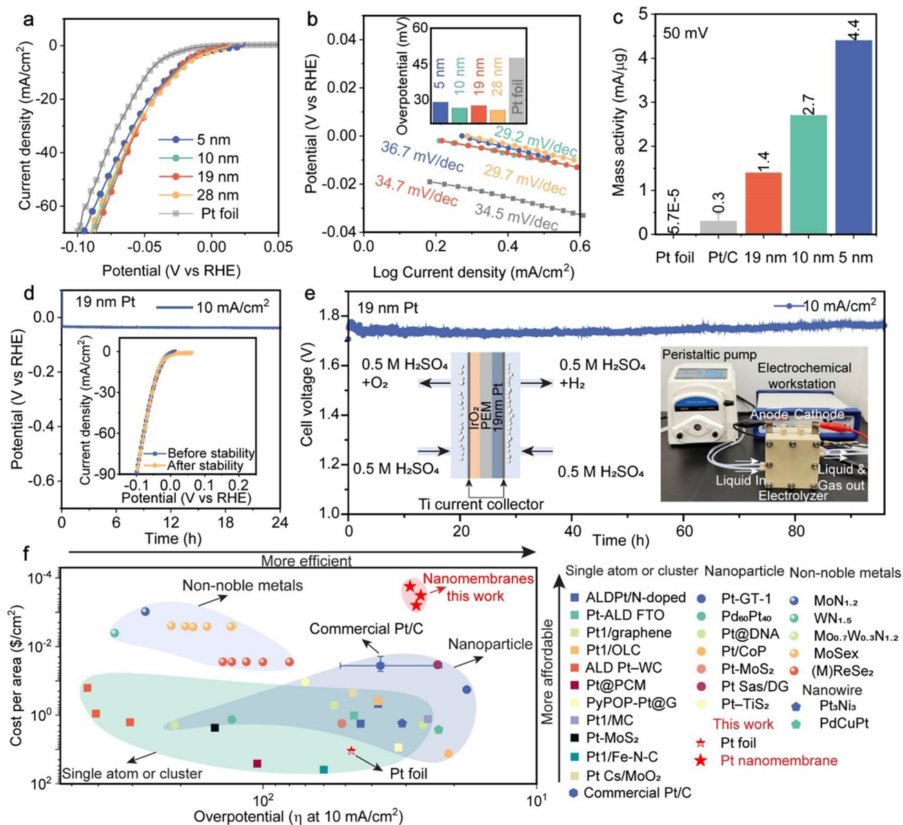
Fig. 3 Acidic HER performance of our Pt nanomembranes. a Linear sweep voltammetry (LSV) curves, b Tafel slopes of 5-nm, 10-nm, 19-nm, 28-nm-thick Pt nanomembrane and bulk Pt foil. The inset shows overpotential at 10 mA cm -2 . c Comparison of mass activities measured at 50 mV for our Pt nanomembranes with those of Pt foil and commercial Pt/C. d Stability tests of 19-nm-thick Pt nanomembrane at the current density of 10 mA cm -2 . e Proton exchange membrane water electrolyzer (PEM-WE) device performance using our 19 nm Pt nanomembrane as the cathodic HER catalyst and Commercial IrO 2 as the anodic OER catalyst at room temperature, insets are the schematic (left) and photograph (right) of the PEM-WE. f Comparison of our Pt nanomembranes and other HER electrocatalysts in terms of overpotential at 10 mA cm -2 and cost per area
