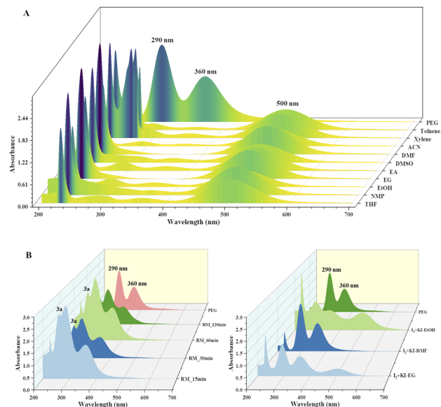
Fig. 2 UV-visible spectrum of (A) various iodine and solvent mixtures depicting the formation of I 3 - anion; peaks at 290 nm and 360 nm for the I 3 - and peak at 500 nm for the I 3 - and KI for I 2 ; (B) formation of I 3 - anion by the reaction of iodine and KI in solvents and in reaction mixture (PEG) at different time intervals.
