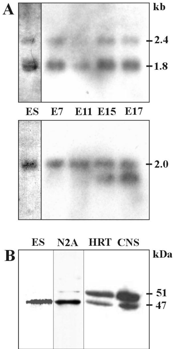
Figure 1 Expression of Annexin A7. (A) Northern blot analysis of RNA from ES-cells and embryos E7, E11, E15, E17 probed with a full length annexin A7 cDNA. Transcripts of 1.8 and 2.4 kb are detected in all stages examined (upper panel). Reprobing with a \beta -actin probe verified equal loading (lower panel, 2.0 kb band). (B) Murine ES cells (ES) express only the small Annexin A7 isoform. Both isoforms are expressed in neuroblastoma neuro-2a cells (N2A), heart (HRT) and brain tissue (CNS) from adult mice. Proteins from neuro-2a and ES cells, heart and brain were resolved by SDS polyacrylamide gel electrophoresis (12% acrylamide) and transferred to nitrocellulose membranes. The Western blot was probed with mAb 203–217 followed by incubation with a peroxidase coupled secondary antibody. Detection was with enhanced chemiluminescence.
