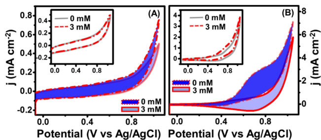
Figure 5. Sensing response study of different catalysts in the absence and presence of glucose: (A) M-AC and (B) \text{Cu}_2\text{O}/\text{M}/\text{AC} (insets of (A) AC and (B) \text{AC}-\text{Cu}_2\text{O} ).
