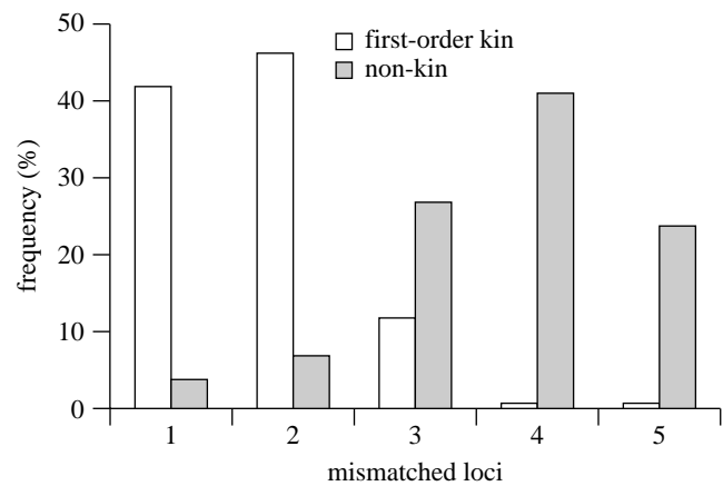
Figure 1. Frequency distribution of the number of mismatches at eight polymorphic loci for 19 helper/breeder pairs known from pedigrees to be close kin and for 30 male and female breeding pair members that were assumed to be non-kin.
