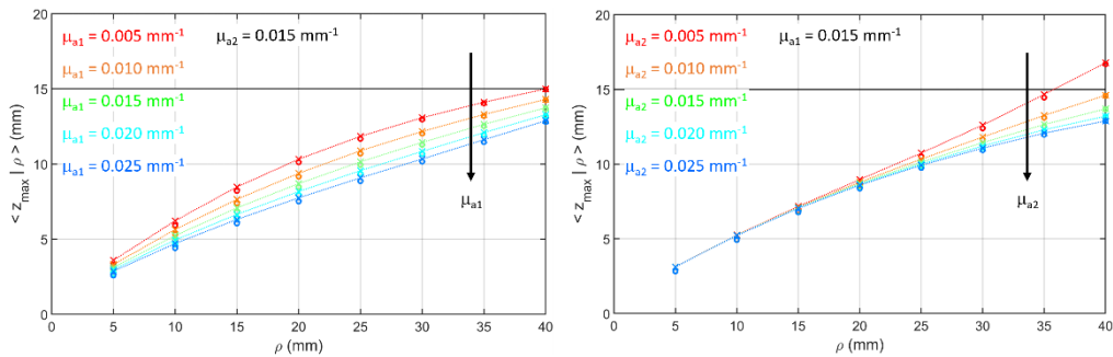
Fig. 9. \langle z_{max}|\rho \rangle as a function of \rho for a two-layer medium ( s_1 = 15 mm, s_2 = 75 mm, n_1 = n_2 = 1.4 , \mu'_{s1} = \mu'_{s2} = 1.0 mm ^{-1} ). (a) variable \mu_{a1} = 0.005, 0.010, 0.015, 0.020, 0.025 mm ^{-1} , fixed \mu_{a2} = 0.015 mm ^{-1} ; (b) fixed \mu_{a1} = 0.015 mm ^{-1} , variable \mu_{a2} = 0.005, 0.010, 0.015, 0.020, 0.025 mm ^{-1} . Circles are DE results, crosses are MC results. Lines connect MC results to guide the eye.
