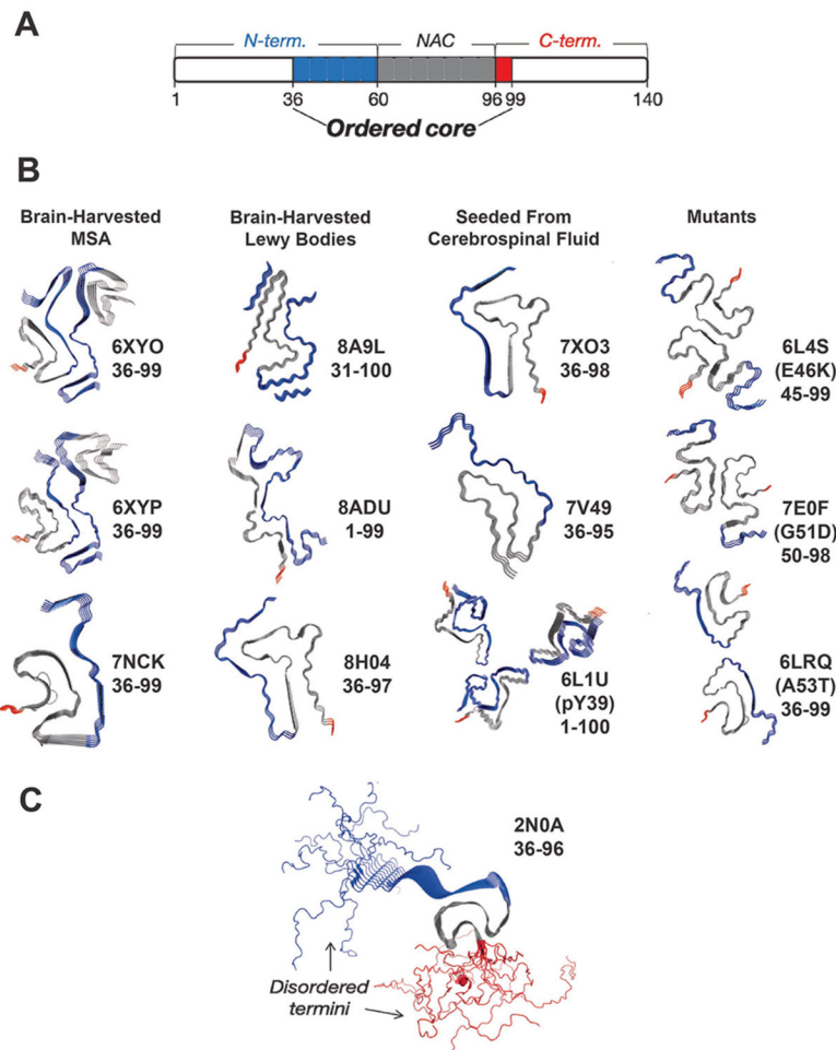
FIGURE 3: The C-terminal domain forms a fuzzy coat on the \alpha -Syn fibril surface (a) Schematic of \alpha -Syn domains and their involvement in the fibril core. Monomer domains are defined as shown at the top of the schematic while the fibril structures reveal an ordered core composed mainly of the residues 36-99 of the N-terminal (blue: 36-60) and the NAC region (grey; 60-96). A very small portion of the core is composed of residues from the C-terminal domain (red: 96-99). The rest of the residues (white) are considered disordered in the fibril structure. (b) Cryo-EM structures (PDB IDs provided) of the ordered cores brain-harvested \alpha -Syn fibrils from MSA, brain-harvested \alpha -Syn fibrils from Lewy bodies, \alpha -Syn fibrils seeded from cerebrospinal fluid and mutant \alpha -Syn [36-44]. The ordered cores as captured consist almost exclusively of residues in the N-terminal (blue) and NAC (grey) domains while the C-terminal (red) domain is rarely included. (c) The ssNMR structure of an \alpha -Syn fibril as performed by Tuttle et al [33]. The N-terminal residues are depicted in blue, and the C-terminal residues are depicted in red. The calculated NMR structure reflects the disordered N- and C-termini.
