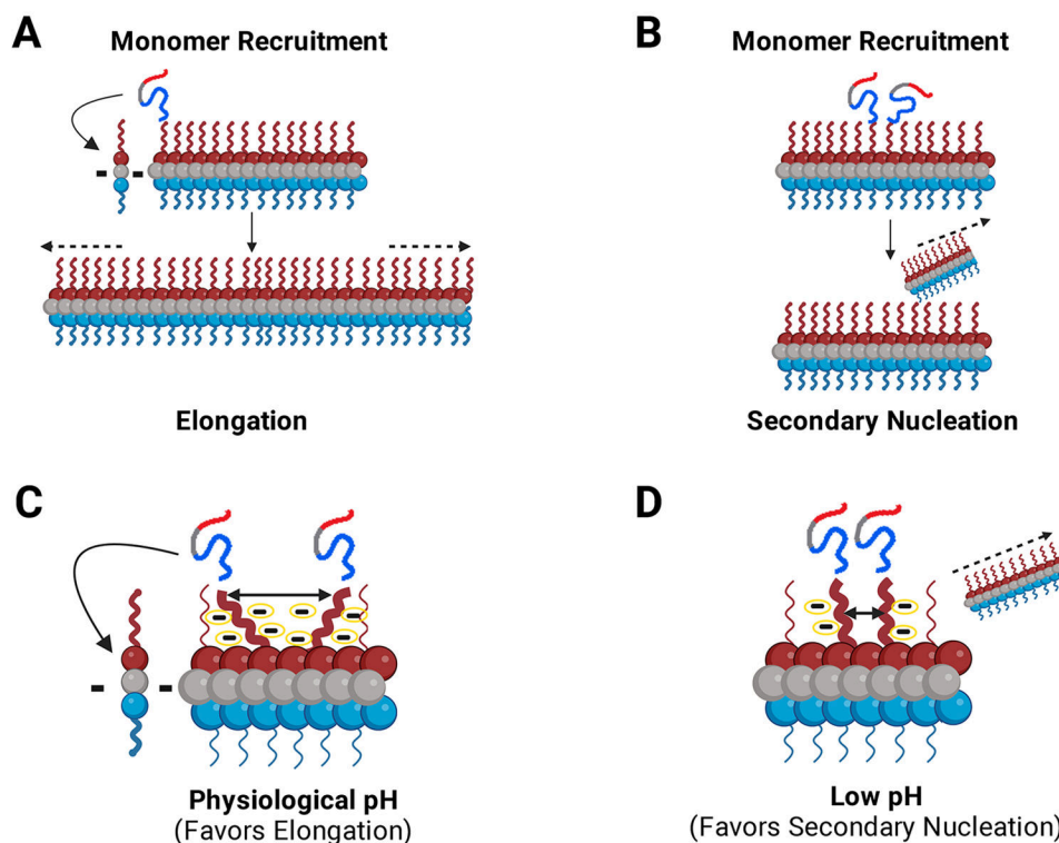
FIGURE 4: Monomers are recruited via the fuzzy coat C-terminal domain for fibril growth and propagation
