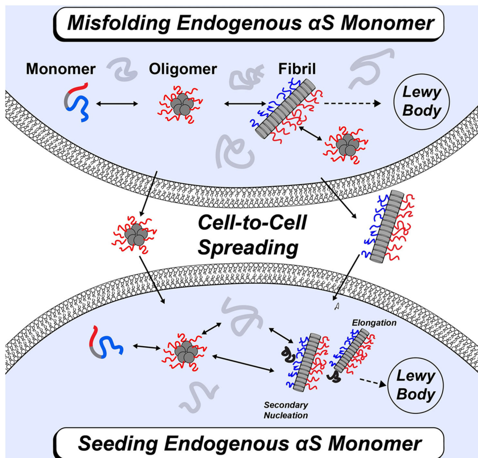
FIGURE 1: Schematic of \alpha -Syn protein aggregation and cell-to-cell spreading (a) Overview of \alpha -Syn aggregation. Endogenous \alpha -Syn monomers (grey) can self-associate into various aggregates including dimers and oligomers. These aggregates can further go on to form different polymorphic amyloid fibrils that can be found in the Lewy bodies of patients with PD. Fibril seeds from one neuron can be released and taken up by a neighboring neuron. This cell-to-cell spreading leads to additional disease progression. (b) Mechanism of \alpha -Syn protein fibril growth and propagation. Endogenous \alpha -Syn monomer can interact with exogenous fibril seeds through elongation and/or secondary nucleation to form mature fibrils.
