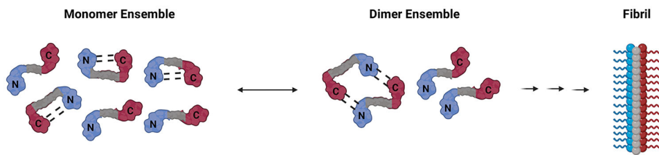
FIGURE 2: Conformational equilibria involved in the early stages of \alpha -Syn aggregation Soluble \alpha -Syn monomers contain a disordered N-terminus (depicted in blue) and a disordered C-terminus (depicted in red). The soluble state monomer ensemble contains various conformations. Specifically, there exist monomers that are in a conformation where the N- and C-terminal domains are close enough to interact with each other. It has been shown in vitro that monomers are in equilibria with a small population of dimers. NMR PRE experiments performed on the monomer-dimer equilibrium revealed the existence of weak transient, but highly specific interactions between N- and C- terminal domains in dimers. Interactions between the termini are shown in dashed lines.
