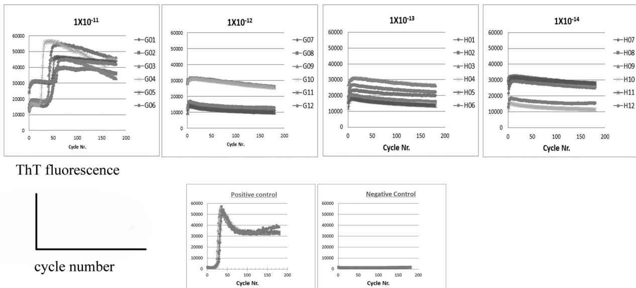
Fig. 1 Analysis of brain tissues from patients with sporadic human prion disease using bioassay and endpoint RT-eQuIC assay. Endpoint RT-eQuIC assay of brain tissue from Patient #1
