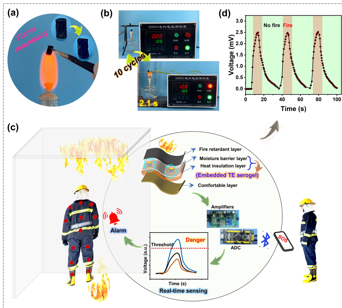
Fig. 6 Aerogel-based self-powered fire warning system. a Flame retardancy property of the aerogel. b Fire warning test for aerogel when exposed to the flame of alcohol lamp. c Schematic showing the aerogel-based self-powered wearable fire warning system that provides high-temperature warning to firefighters. d Voltage curve of aerogel-based self-powered wearable device in three cyclic fire warning tests
