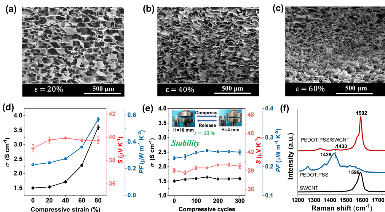
Fig. 2 Microstructure and TE properties of the aerogels. a–c SEM images of TE composite aerogel under different compression strains ((a) \varepsilon=20\% , (b) \varepsilon=40\% , (c) \varepsilon=60\% ). d The TE properties variations when subjected to compression strain (0–80%). e The variation in TE properties for the aerogel after multiple compression cycles with 60% strain. f Raman spectra of the pure SWCNT, PEDOT:PSS and the composite aerogel
