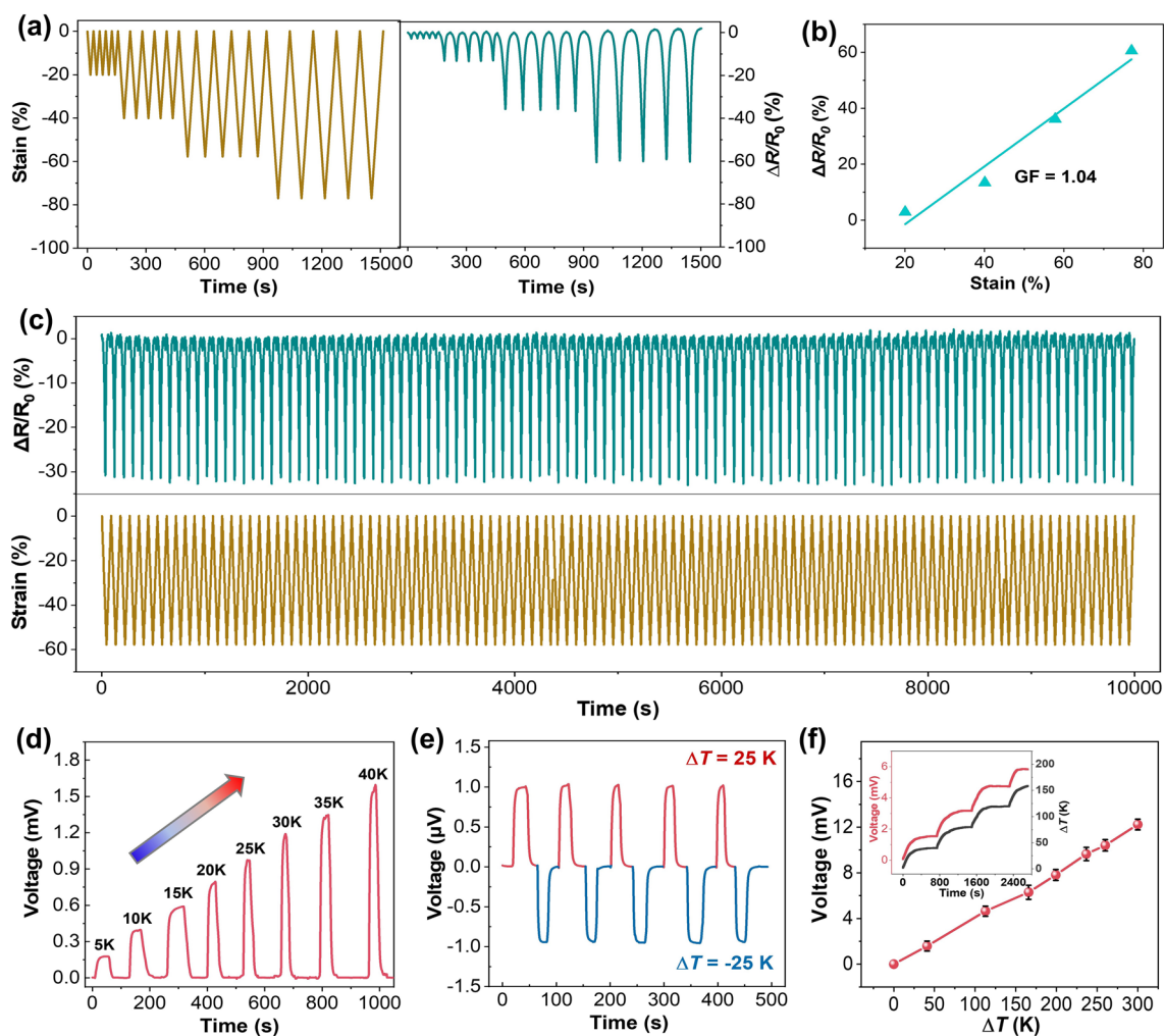
Fig. 3 An aerogel-based temperature and pressure dual-mode sensor. a Real-time relative resistance change ( \Delta R/R_0 ) response of the aerogel subjected to various compression strains. b The \Delta R/R_0 of the aerogel as a function of strain. c The durability test under cyclic loading of 60% strain. d Real-time voltage responses of the aerogel at different \Delta T . e Real-time voltage response of the aerogel under alternating and opposite temperature differences ( \Delta T = \pm 25 K). f The generated voltage as a function of \Delta T , where the inset shows the real-time voltage response to the applied \Delta T
