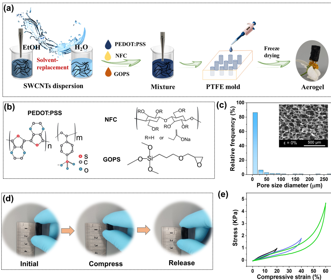
Fig. 1 Aerogel preparation and mechanical properties evaluation. a Schematic illustration of the preparation process of the elastic PEDOT:PSS/SWCNT composite aerogel. b Chemical structures of PEDOT:PSS, NFC and GOPS. c Pore size diameter distribution of aerogel based on mercury injection measurement. Inset of Fig. shows the SEM image of the aerogel. d The digital images depict the states of the aerogel: before (left), during (middle), and after (right) finger pressing. e Compressive stress–strain curves of TE aerogel at different compressive stains
