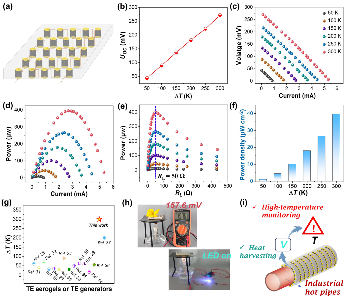
Fig. 4 An aerogel-based TE generator. a Illustration showing the TE generator consisting of 25 aerogels in series. b Open-circuit voltages generated by the aerogel-based TE generator under different \Delta T . c The relationship between the generated output voltage as a function of circuit current at different \Delta T . Output power of TE generator as a function of d circuit current and e external load resistance under different \Delta T . f The power density of the TE generator at different \Delta T . g The comparison of the highest testing temperatures for most TE aerogels and their generators reported in the literature. h Photographs showing the generated voltage or powering a LED by harvesting alcohol lamp flame heat energy. i Illustration showing the high-temperature application scenario of the aerogel-based TE generator by utilizing heat energy on industrial hot pipes
