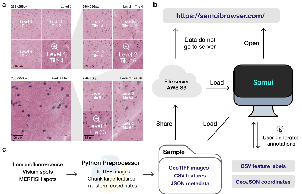
Figure 1. Overview of the Samui. (a) Input images are stored in a tiled GeoTIFF file format. When a user opens the browser, at the lowest zoom setting, only tiles from level 0 are downloaded. With increasing Zoom setting, tiles from increasing levels within the field of view are downloaded as needed. (b) Samui is statically served and relies completely on the client machine for all functionalities. It can load files from a cloud storage link or from the local machine. (c) Samui takes in a Sample folder that contains chunked images, CSV features, and JSON metadata. These are generated with the Python preprocessor and the browser also supports user-generated annotations.
