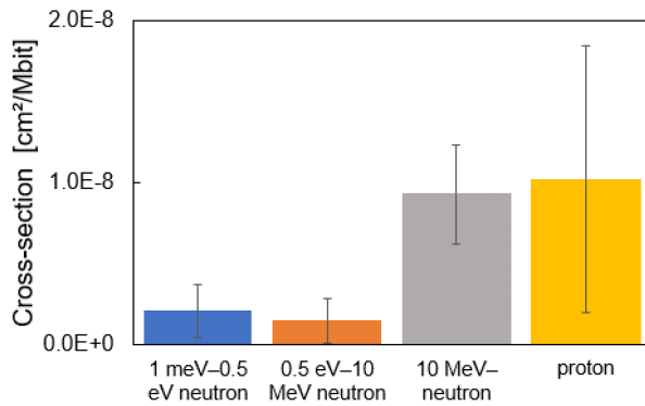
Fig. 6. Results of multiple regression analysis. Cross-sections are shown for each particle type. Error bars indicate standard deviation. In this study, cross-section is defined as the probability of soft errors per megabit (Mbit).
