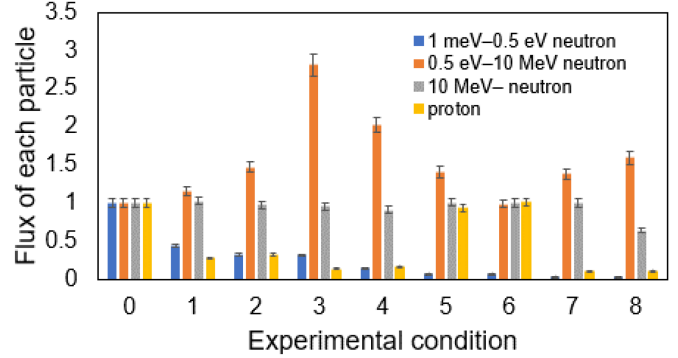
Fig. 4. Radiation quality with each condition normalized with condition 0, in which only acrylic was used. Blue: thermal neutrons (1 meV–0.5 eV), Orange: intermediate-energy neutrons (0.5 eV–10 MeV), Gray: high-energy neutrons ( >10 MeV), and Yellow: protons. The error bars indicate the error considering error propagation as a ratio to condition 0.
