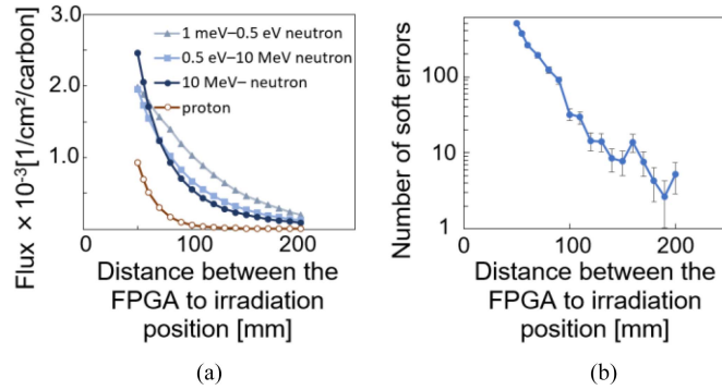
Fig. 3. Secondary particle distribution calculated via PHITS simulation (a), and the number of soft errors generated with varying distances from the irradiation position (b). Error bars indicate standard deviation.
