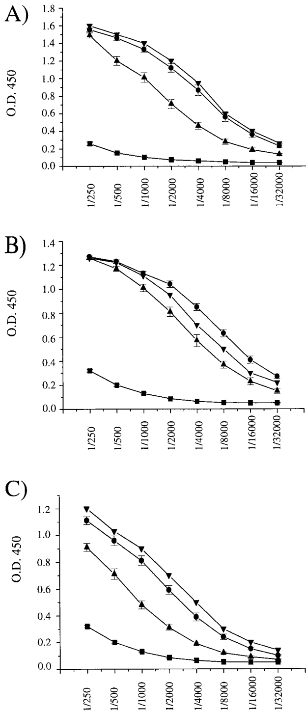
FIG. 8. Anti-Ad antibodies in CBA/J mice. Mice were injected intravenously with 10^9 IU of AdE1 ^\circ (A) and AdE1 ^\circ E4 ^\circ (C) and 10^9 PFU of AdE1 ^\circ E2A ^\circ (B) vectors. Sera were collected at days 4 (■), 35 (▲), and 90 (●) postinjection and analyzed by ELISA as previously described (37). Data are expressed as the means of the optical density at 450 nm (O.D. 450) \pm SE determined for successive serial dilutions of the sera recovered from 5 to 10 mice per experimental group. Each plate contained the same positive control serum (▼).
