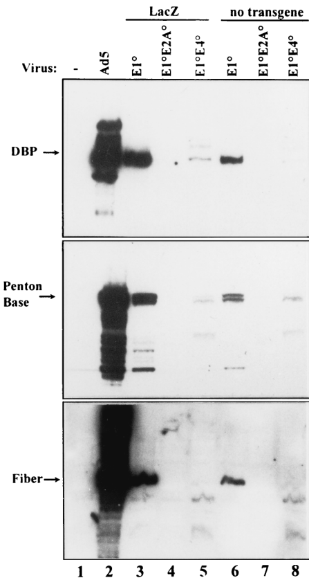
FIG. 4. Expression of early and late viral proteins in noncomplementing human A549 cells. A549 cells were infected with the indicated vectors at an MOI of 500 BU/cell (lanes 3, 4, and 5) or 500 IU/cell (lanes 6, 7, and 8). Wild-type Ad5 was infected with an MOI of 0.5 IU/cell. At 72 h p.i. total protein was extracted and processed as described in the legend to Fig. 1.
