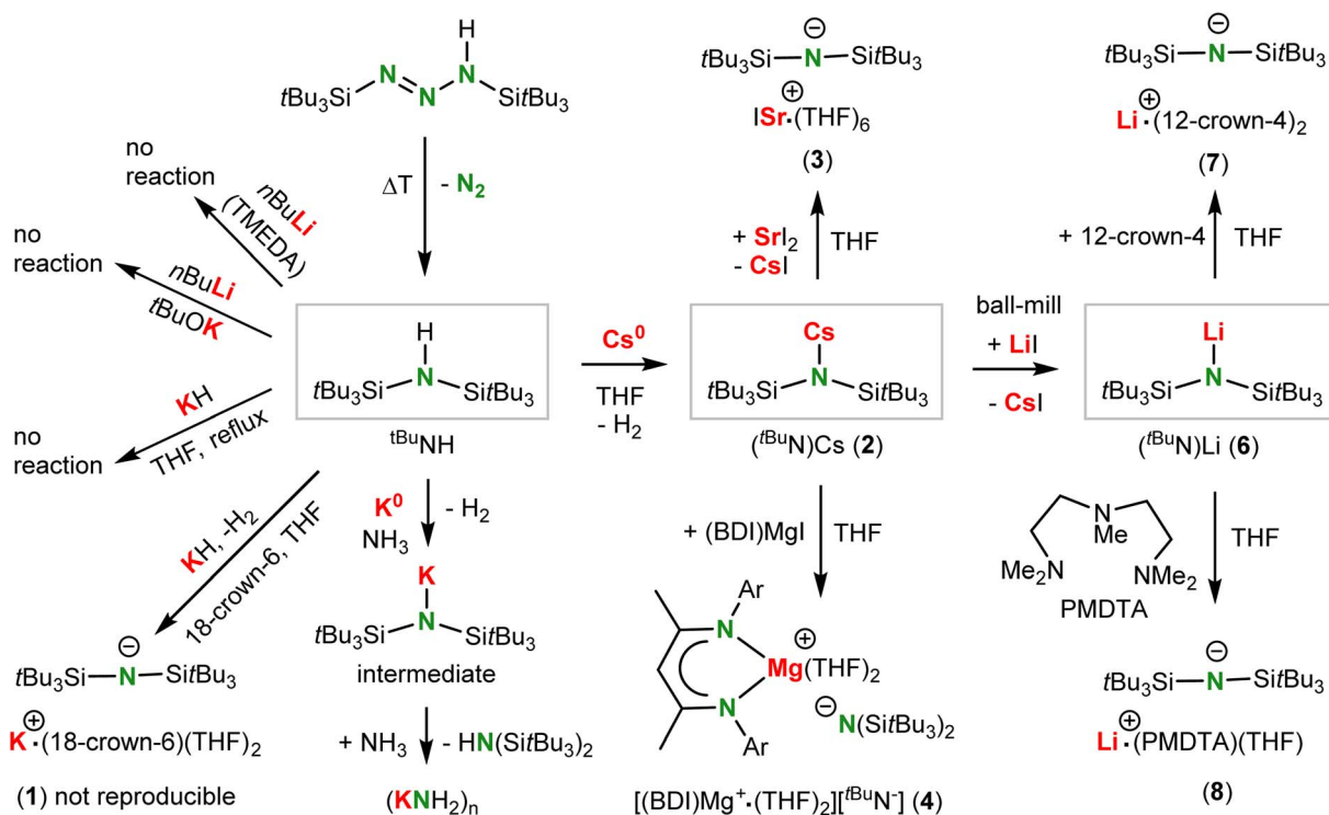
Scheme 2 Synthesis and deprotonation of {}^t\text{Bu}_3\text{NH} and complexes with the bulky {}^t\text{Bu}_3\text{N}^- anion.
