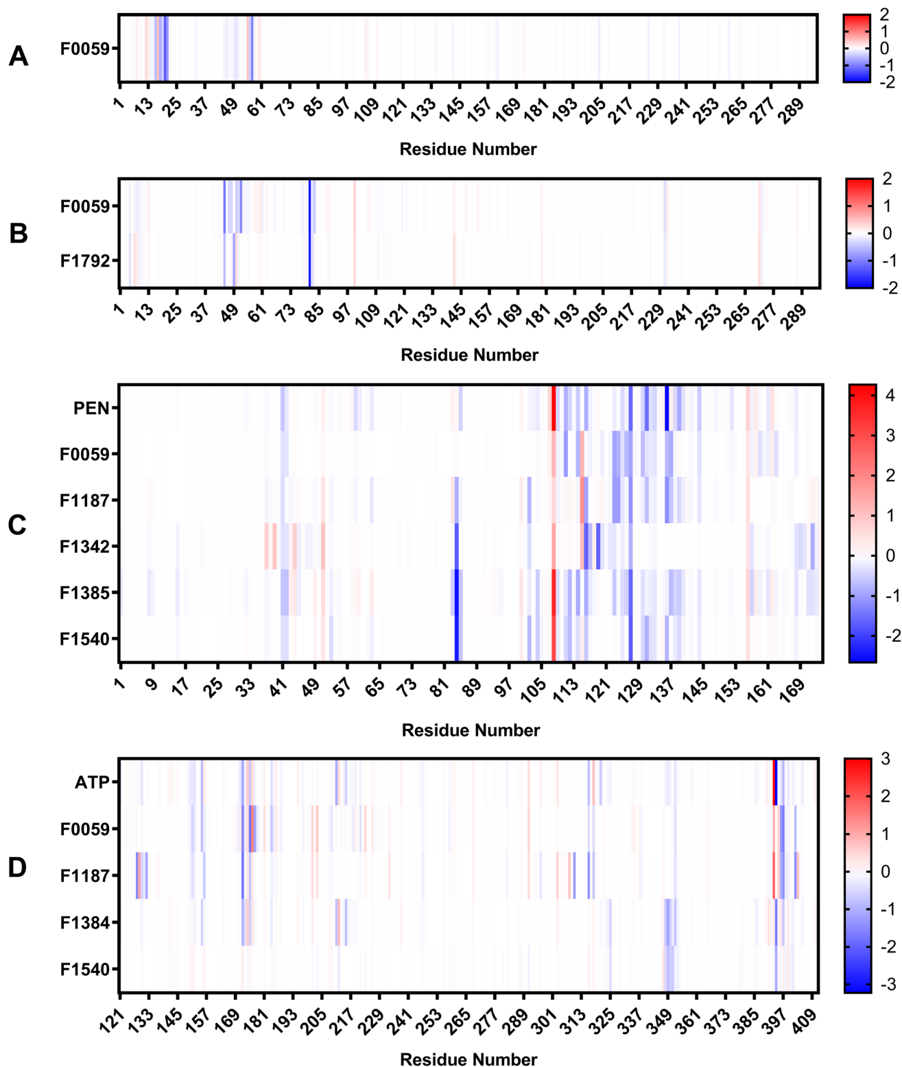
Fig. 5 Binding energy contribution of the protein residues. Values are in \text{kcal mol}^{-1} (A) ASFVAP_R1 (B) ASFVAP_R3 (C) ASFVProIX (D) ASFVlig. Blue streaks represent attractive interactions, while red streaks represent repulsive interactions.
