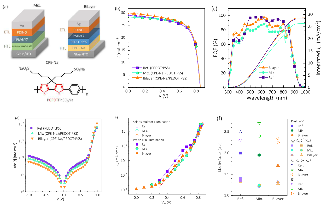
Figure 3. (a) Schematic structure of the studied devices and optoelectronic characterization: illustrative (b) current density–voltage measured with solar simulator; (c) external quantum efficiency; (d) dark current–voltage curves; (e) short-circuit current versus open-circuit current for different illumination conditions, as indicated; and (f) summary of ideality factors.
