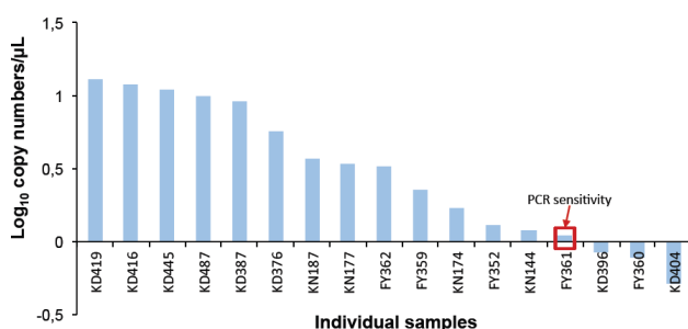
Figure 1. RT-qPCR sensitivity shown by log results of each individual sample.
