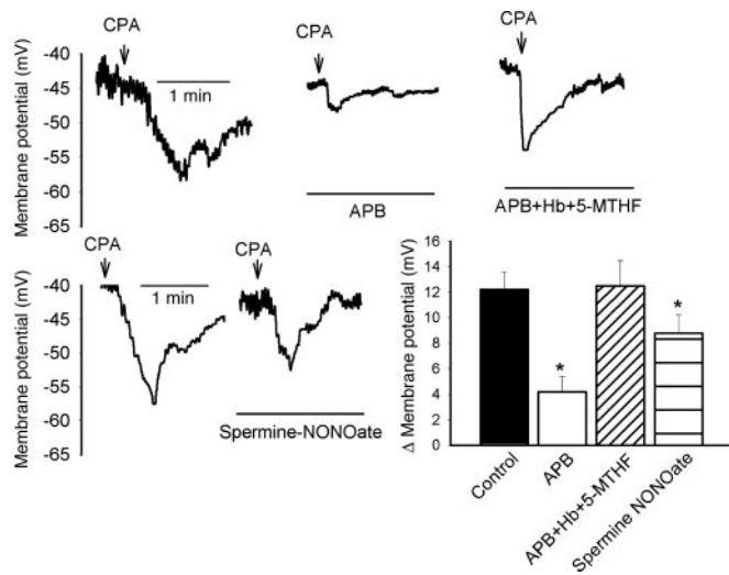
Fig. 4. Original recordings and histogram showing that the ability of 100 \mu\text{M} 5-MTHF to prevent inhibition of CPA-evoked subintimal hyperpolarization by 10 \mu\text{M} APB was not diminished to 10 \mu\text{M} hemoglobin, and that 10 \mu\text{M} spermine-NONOate depressed the hyperpolarizing response to CPA without altering resting membrane potential. *, P < 0.05 , compared with control.
