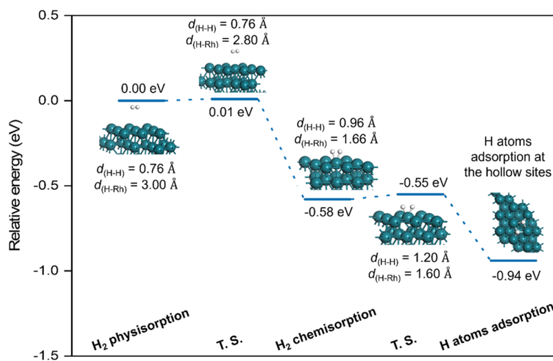
Figure 2. ZPE-corrected relative energies and the structures for the processes of H 2 adsorption and dissociation. The transition states (T.S.) for H 2 dissociative adsorption and H diffusion processes are also shown here. d_{(\text{H-H})} and d_{(\text{H-Rh})} represent the H–H distance and H–Rh distance, respectively. The teal and white spheres are the Rh and H atoms, respectively. The zero-energy state corresponds to physisorbed H 2 .
