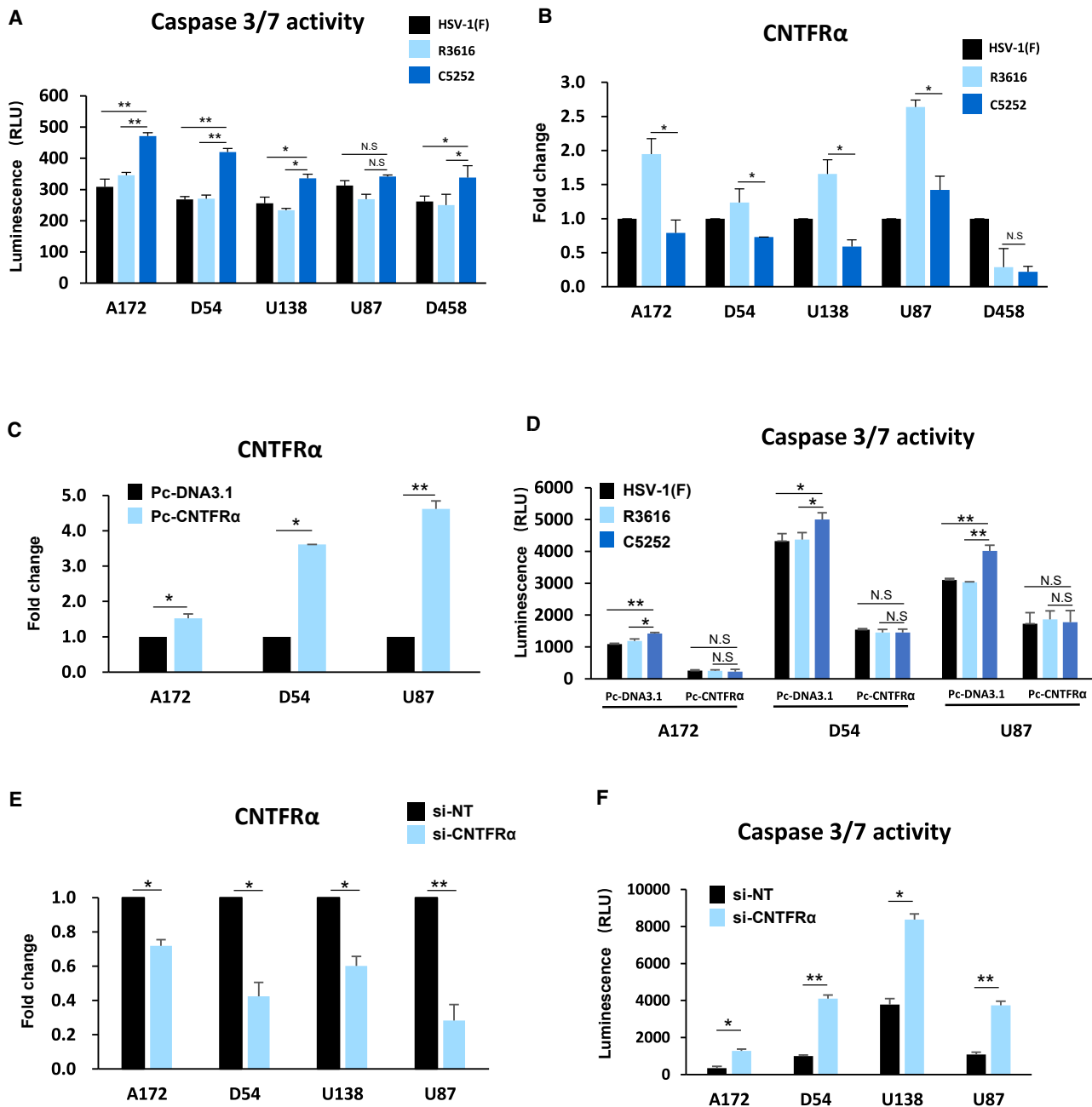
Figure 3. Caspase-3/7 activity and CNTFRα expression during C5252 infection in glioblastoma cells
