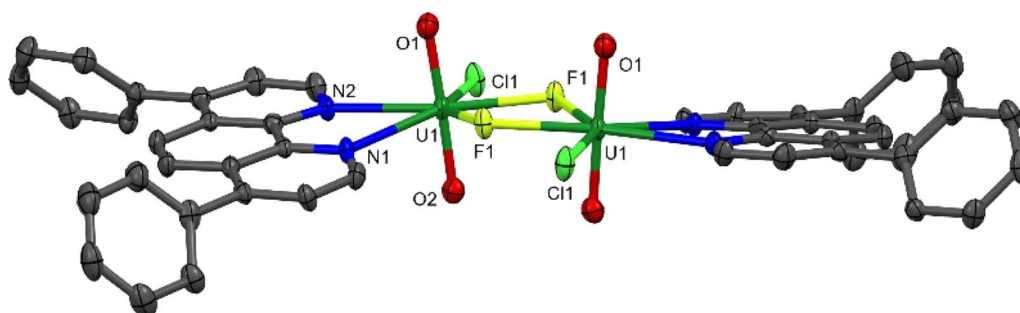
Fig. 11 Solid-state structure of [\text{UO}_2\text{ClF}(\text{Ph}_2\text{phen})]_2 [\mathbf{1-Cl-F}]_2 with thermal ellipsoids at the 50% probability level. Hydrogen atoms are omitted for clarity.
