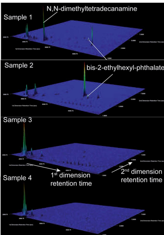
Fig. 4. Extracted ion chromatograms ( m/z 41) illustrate detection of N,N -dimethyltetradecylamine and bis-2-ethylhexyl phthalate using GC \times GC-TOF-MS in high DRO samples (1 and 2) and no detection in low DRO samples (3 and 4). Mass spectra of samples 1, 2, and the bis-2-ethylhexyl phthalate standard are given in the ESI (Fig. S5 † ). N,N -dimethyltetradecanamine identification was also confirmed with an authentic standard. These signals were absent in 14 field and lab blanks, and absent in two field blanks collected at the same time and two lab blanks extracted on the same date as samples 1 and 2 (Fig. S5 † ). The z -axis is scaled automatically to the highest intensity peak. The color map indicates the extracted ion intensity (where the maximum height is colored red) and the small peaks (colored royal blue) are close to the baseline intensity due to their small abundance.
