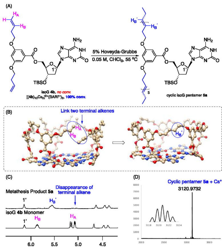
Figure 3. Chemical structure, model and characterizations of cyclic doxy isoG pentamer 5a . (A) Macrocyclization process through olefin metathesis; (B) Computational model of cyclic pentamer; (C) ^1\text{H} NMR spectra of deoxy isoG 4b monomer and metathesis product cyclic doxy isoG pentamer 5a in DMSO; (D) MALDI-TOF spectrum showing the effective extraction of \text{Cs}^+ from aqueous phase.
