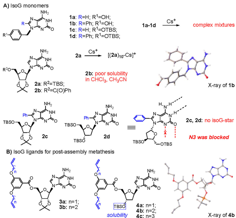
Figure 1. (A) Non-sugar IsoG derivatives 1 and 8-phenyl-isoG derivatives 2 ; (B) IsoG ligand 3 and 4 for post-assembly weaving.
