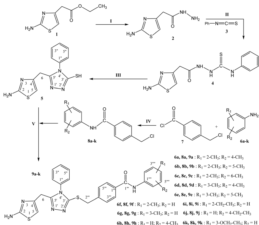
Scheme 1 Outline for the synthesis of 4-(((5-((2-amino-1,3-thiazol-4-yl)methyl)-4-phenyl-4H-1,2,4-triazol-3-yl)sulfanyl)methyl)-N-(aryl) benzamides. Reagents & conditions: (I) MeOH/N 2 H 4 ·H 2 O/refluxing for 2 h (yield = 91%). (II) MeOH/3/refluxing for 1 h (yield = 88%). (III) The ppt. of 4 dissolved in 10% NaOH/filtration/acidification of filtrate in cold state to get ppt. of 5 (yield = 87%). (IV) Aqueous Na 2 CO 3 solution/pH 9–10/vigorous manual shaking at RT for 2–3 h (yield = 89%). (V) DMF/LiH/stirring for 12–24 h (yield = 92–98%).
