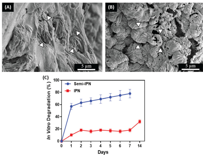
Fig. 4. Microstructure and in vitro degradation of semi-IPN and IPN GelMA/pectin-g-PCL hydrogels. Representative SEM images of (A) semi-IPN hydrogels synthesized using 10% GelMA, and 1.15% pectin-g-PCL, and (B) IPN hydrogels synthesized using 10% GelMA, 1.15% pectin-g-PCL, and 0.5% Ca 2+ . White arrows indicate pectin-g-PCL aggregates within the GelMA network. (C) In vitro degradation rate of semi-IPN and IPN GelMA/pectin-g-PCL hydrogels.
