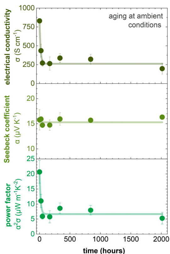
Figure 4. Electrical conductivity \sigma , Seebeck coefficient \alpha , and power factor \alpha^2\sigma versus aging time of p(g_32T-T) coprocessed with 20 mol % of F_4TCNQ at ambient conditions; error bars represent the standard deviation of five measurements on the same sample.
