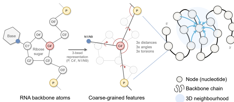
Figure 2: gRNAde featurizes RNA backbone structures as 3D geometric graphs. Each RNA nucleotide is a node in the graph, consisting of 3 coarse-grained beads for the coordinates for P, C4', N1 (pyrimidines) or N9 (purines) which are used to compute initial geometric features and edges to nearest neighbours in 3D space. Backbone chain figure adapted from Ingraham et al. (2019) .
