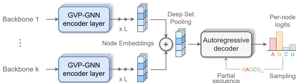
Figure 12: gRNAde model architecture. One or more RNA backbone geometric graphs are encoded via a series of SE(3)-equivariant Graph Neural Network layers (Jing et al., 2020) to build latent representations of the local 3D geometric neighbourhood of each nucleotide within each state. Representations from multiple states for each nucleotide are then pooled together via permutation invariant Deep Sets (Zaheer et al., 2017), and fed to an autoregressive decoder to predict a probabilities over the four possible bases (A, G, C, U). The probability distribution can be sampled to design a set of candidate sequences. During training, the model is trained end-to-end by minimising a cross-entropy loss between the predicted probability distribution and the true sequence identity.
