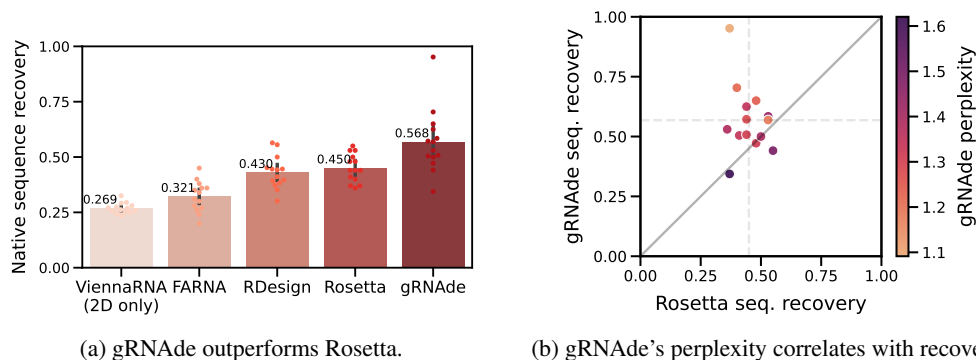
Figure 4: gRNAde compared to Rosetta for single-state design. (a) We benchmark native sequence recovery of gRNAde, RDesign, Rosetta, FARNA and ViennaRNA on 14 RNA structures of interest identified by Das et al. (2010) . gRNAde obtains higher native sequence recovery rates (56% on average) compared to Rosetta (45%) and all other methods. (b) Sequence recovery per sample for Rosetta and gRNAde, shaded by gRNAde's perplexity for each sample. gRNAde's perplexity is correlated with native sequence recovery for designed sequences (Pearson correlation: -0.76, Spearman correlation: -0.67). Full results on single-state test set are available in Appendix B and per-RNA results in Appendix Table 2 .
