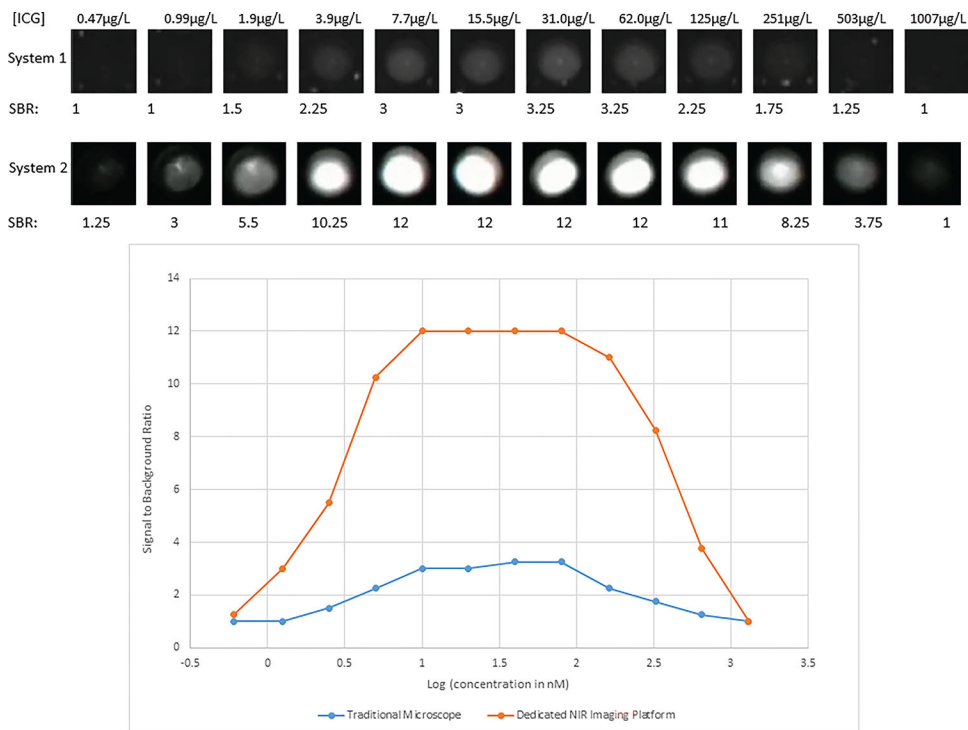
Figure 2. Comparing NIR sensitivity of a dedicated NIR detector and an add-on detector to pre-existing microscope. Above) Serial dilutions of ICG ranging from 0.47µg/L - 1007µg/L. The same plates were imaged using the Leica platform and the VisionSense platform. Below each well is the signal to background ratio of the corresponding well in the respective visualization systems. An SBR = 1 shows that the fluorescence signal is the same as background == black. Below) Plot of SBR vs log concentration ranging from 1.30µM – 0.6nM. The SBR peaks near 3 for System 1 and 12 for System 2. At concentrations above 80nM, there is auto-quenching of the fluorophores.
