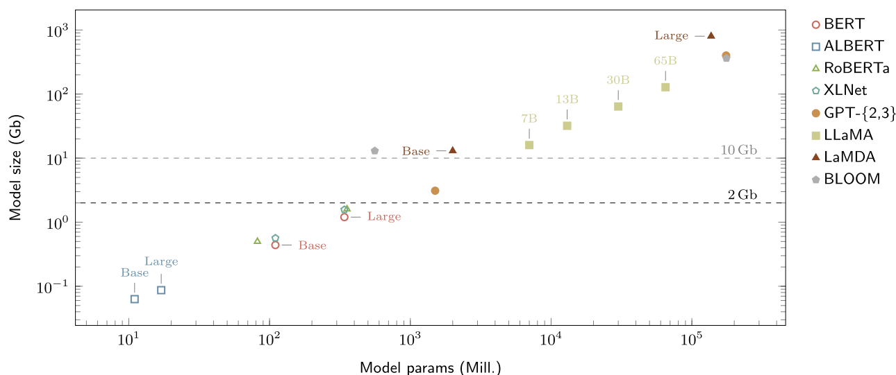
Figure 1. Overview of some popular LLMs. Axes are in logarithmic scale to ease the visualization (almost a linear relationship between model size and model parameters). Each model has different variants available, such as Base and Large (see the plot annotations). As discussed in the next section, we set 2 Gb as the upper-bound for LLM size so that it can be deployed on commodity mobile and ubiquitous devices (see 'Models' section for more details). Therefore, in this paper, only the models below such an upper-bound are considered lightweight .
