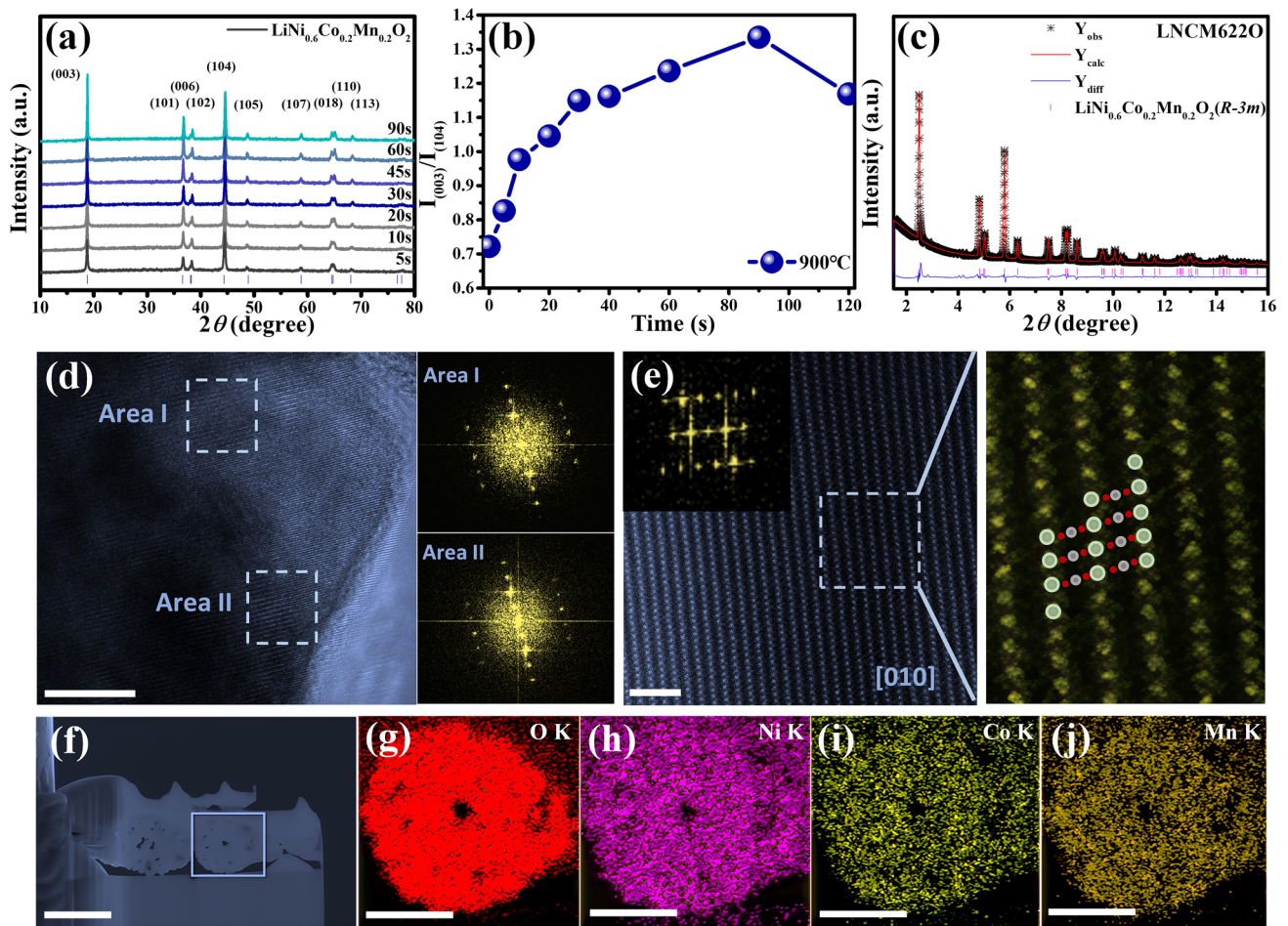
Fig. 3 Synthesis, structural characterization of the synthesized \text{LiNi}_{0.6}\text{Co}_{0.2}\text{Mn}_{0.2}\text{O}_2 cathode materials. a Ex situ XRD patterns evolution of NCM622 in the HTS process at 900\text{ }^\circ\text{C} . b Evolution of the cationic disordering. c Refined X-ray diffraction pattern of 900\text{ }^\circ\text{C} , 90-s sample. The sample consists of the layered R\bar{3}m (Li-TM-O 2 ). d TEM image for 900\text{ }^\circ\text{C} , 90-s sample, scale bar, 10 nm. The inset images are the fast Fourier transform pattern for the TEM image. e HAADF-STEM image, scale bar, 2 nm, corresponding atomic mode. f–j FIB image, scale bar, 2.5 \mu\text{m} and EDX elemental mapping of O, Ni, Co, and Mn cross-section of secondary particle for pristine NCM622 cathode, scale bar, 1 \mu\text{m}
