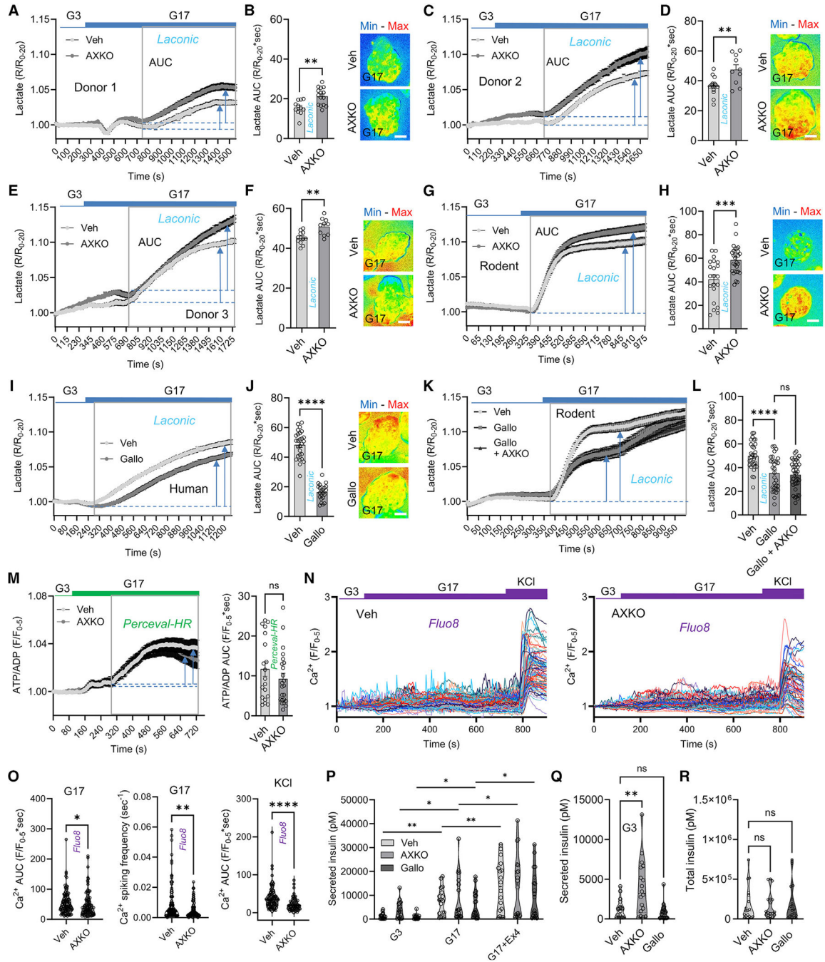
Figure 4. Effects of LDHB inhibition on lactate levels and function in human \beta cells (A–F) Traces (A, C, and E) and bar graph and representative images (B, D, and F) showing that glucose-stimulated lactate generation is amplified by 10 \mu M AXKO-0046 (LDHB inhibitor) in islets from three separate donors (donor 1, n = 10 –15 islets; donor 2, n = 10 –14 islets; donor 3, n = 10 –12 islets) (unpaired t test). (G and H) AXKO-0046 amplifies glucose-stimulated lactate generation in mouse \beta cells, as shown by mean traces (G) and summary bar graph and representative image (H) ( n = 21 –28 islets, three animals) (unpaired t test).
