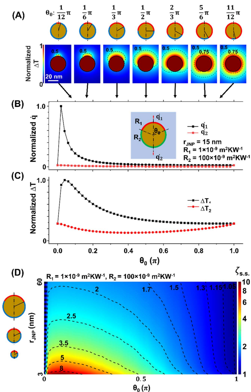
Fig. 3 Effect of the polar angle ( \theta_0 ) on the temperature contrast under steady-state. (A) Temperature profile of JNP heating with different \theta_0 . R_1 = 1 \times 10^{-9} \text{ m}^2 \text{ K W}^{-1} and R_2 = 100 \times 10^{-9} \text{ m}^2 \text{ K W}^{-1} , r_{JNP} = 15 nm. (B) The local heat flux rate across the interface at the northern pole ( \dot{q}_1 ) and southern pole ( \dot{q}_2 ) as a function of \theta_0 . (C) \Delta T_1 and \Delta T_2 as a function of \theta_0 . (D) \zeta_{s.s.} map as a function of r_{JNP} and \theta_0 . R_1 = 1 \times 10^{-9} \text{ m}^2 \text{ K W}^{-1} , R_2 = 100 \times 10^{-9} \text{ m}^2 \text{ K W}^{-1} . The dotted lines are contour lines for \zeta_{s.s.} .
