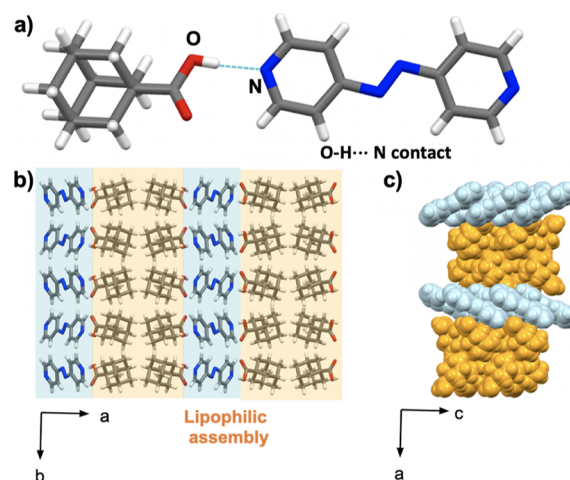
Figure 2. X-ray crystal structure of 2( ada )·( azop ): (a) molecular units sustained by [\text{O}-\text{H}\cdots\text{N}] hydrogen bonds, (b) lipophilic assemblies of cocrystal aggregates in the ab -plane, and (c) spacefill view of level sheets along the c -axis.
