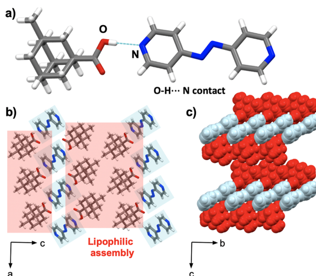
Figure 3. X-ray crystal structure of 2( dimet-ada )·( azop ): (a) molecular units sustained by [\text{O}-\text{H}\cdots\text{N}] hydrogen bonds, (b) lipophilic assemblies of cocrystal aggregates in the ac -plane, and (c) spacefill view of corrugated sheets along the b -axis.
