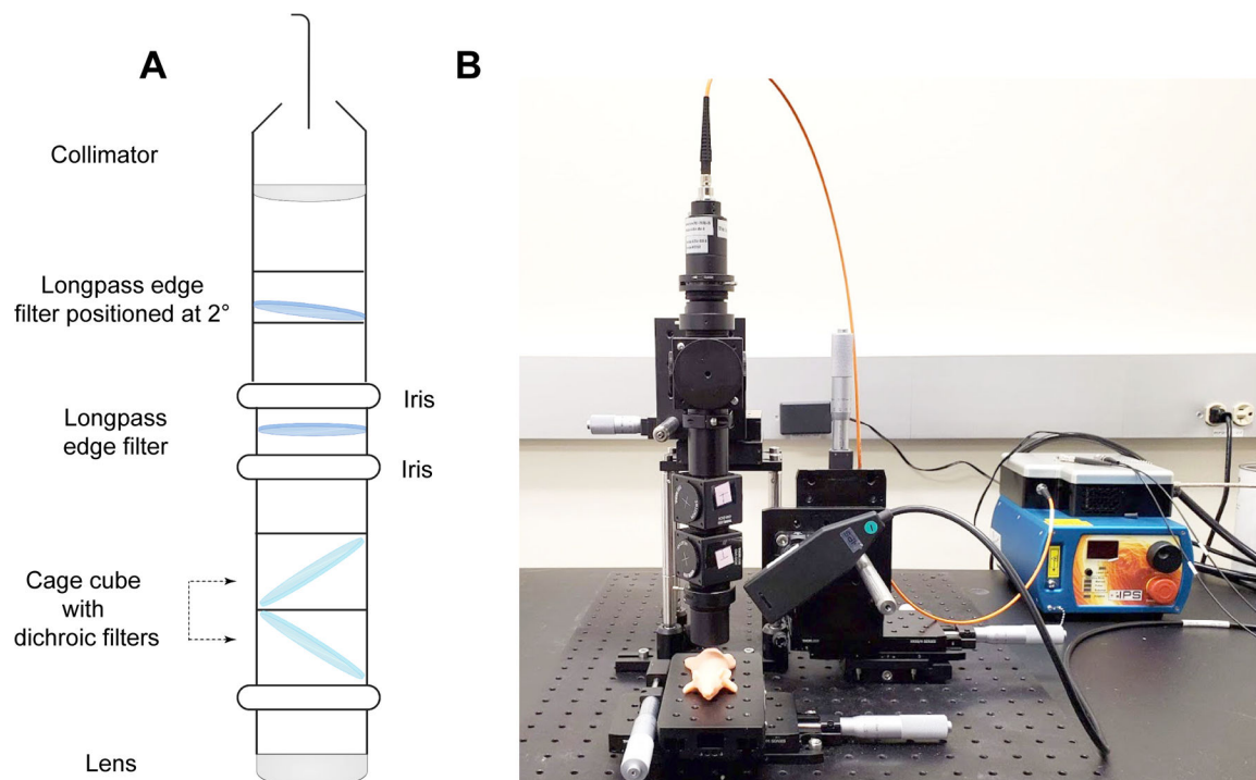
Fig. 1 | SORS Set-up using the custom-built probe.
