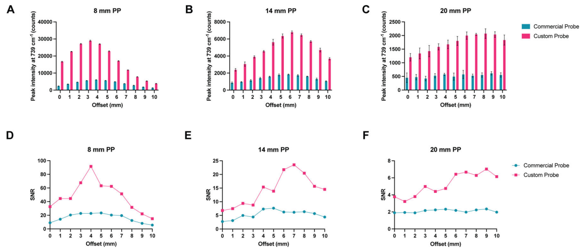
Fig. 2 | Comparison of the collection efficiencies of the commercially available collection probe and the custom-built collection probe.
