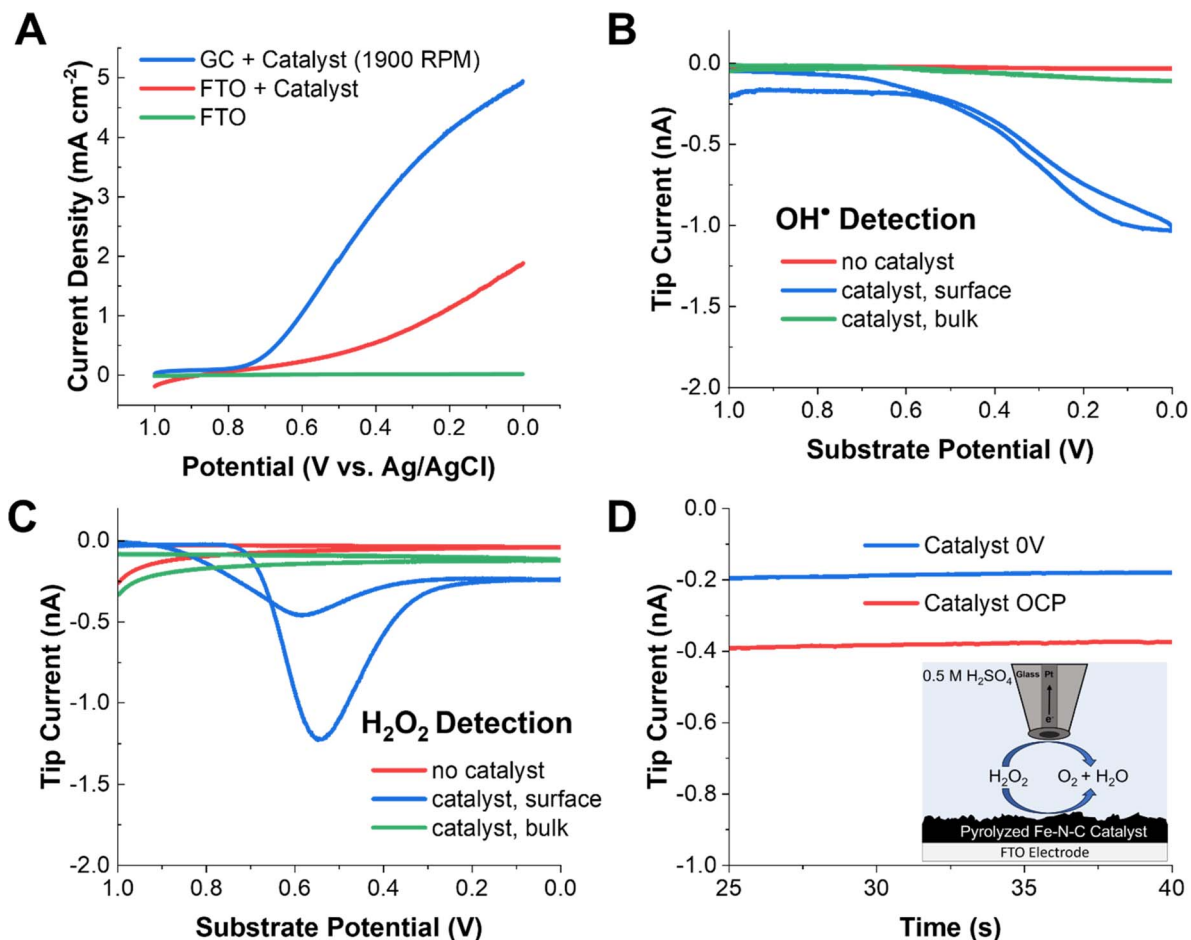
Fig. 1 SECM results for radical and H 2 O 2 detection on pyrolyzed Fe–N–C catalysts. (A) Substrate LSVs of the catalyst on a rotating GC electrode and a stationary FTO substrate in oxygen-saturated 0.5 M H 2 SO 4 , as well as a catalyst-free FTO blank. (B) The radical SG/TC response at the gold tip as the substrate potential is swept at 10 mV s −1 with 25 mM DMPO in solution. (C) The H 2 O 2 SG/TC response on a Pt tip as the substrate potential is swept at 10 mV s −1 . (D) Redox competition mode SECM with a Pt tip located above the Fe–N–C in 0.5 mM H 2 O 2 solution in 0.5 M H 2 SO 4 purged with argon, with the substrate biased to the ORR and under open circuit conditions.
