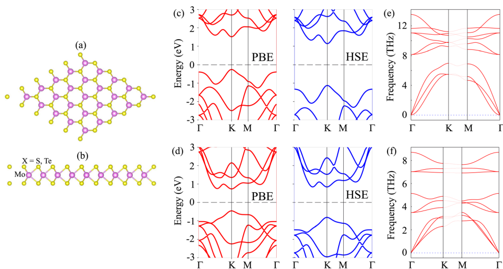
Fig. 1 (a) Top view and (b) side view of the atomic structures of a MoX 2 (X = S, Te) monolayer. Calculated electronic band structures of (c) MoS 2 and (d) MoTe 2 monolayers from PBE and HSE functionals. Phonon spectrum of (e) MoS 2 and (f) MoTe 2 monolayers.
