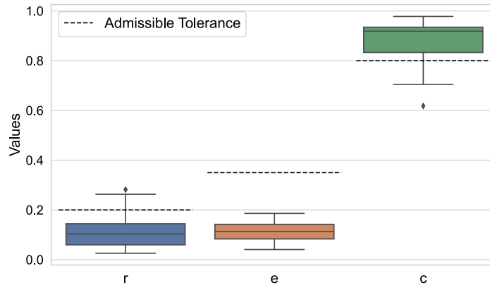
Fig. 15. Distribution of error assessment metrics.
