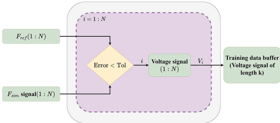
Fig. 10. Voltage training buffer update.
