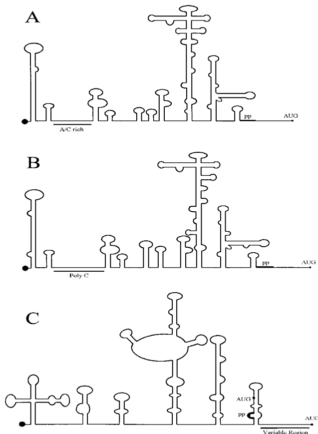
FIG. 2. (A) Schematic representation of the predicted 5'UTR secondary structure of the parechovirus HPEV1. The structure is strikingly similar to that predicted for encephalomyocarditis virus (B), a representative of the cardio- and aphthovirus 5'UTR group; it is dissimilar from that of poliovirus (C), a representative of the entero- and rhinovirus 5'UTR group. All picornaviruses have a polypyrimidine tract (shown as a heavy line and labelled pp) about 20 nucleotides upstream of an AUG (labelled with a square). In cardio- and aphthoviruses this AUG initiates the open reading frame, while in entero- and rhinoviruses a second AUG located downstream has this function. The variable region is seen in all enteroviruses, but is largely deleted in rhinoviruses. VPg, covalently attached to the 5' terminus, is shown as a solid circle.
