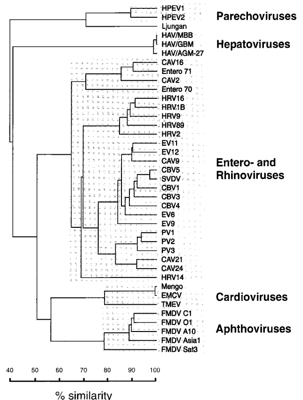
FIG. 3. Dendrogram, based on comparisons of the VP3 protein, illustrating the genetic relationships among selected representatives of each of the picornavirus genera. Abbreviations: HAV, hepatitis A virus; HRV, human rhinovirus; EV, enterovirus; CBV, coxsackie B virus; SVDV, swine vesicular disease virus; PV, poliovirus; EMCV, encephalomyocarditis virus; TMEV, Theiler's murine encephalomyelitis virus; FMDV, foot-and-mouth disease virus.
