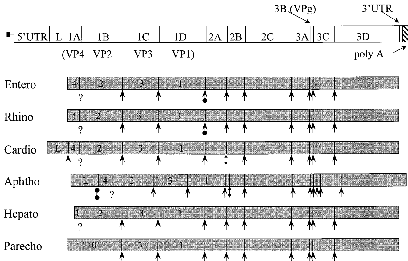
FIG. 1. The genome of a typical picornavirus, together with schematic maps of the polyprotein in each of the six picornavirus genera. VPg, the peptide covalently attached to the 5' terminus of the RNA genome, is shown as a small solid square. The virus-encoded activities responsible for processing each protein boundary are indicated: vertical arrows, 3C pro cleavages (also including those for which 3CD pro are required); arrow with circle, 2A pro , the trypsin family member found in enteroviruses and rhinoviruses; double-headed arrow, 2A-associated cleavages in cardioviruses and aphthoviruses; barbell, L pro of aphthoviruses. The site of VP0 (maturation) cleavage, which occurs by an unknown, possibly autocatalytic mechanism, is indicated (?). For clarity, the positions of VP4 (1A), VP2 (1B), VP3 (1C), VP1 (1D), and VP0 (1AB) are indicated on the polyprotein maps as 4, 2, 3, 1, and 0, respectively. The aphthovirus foot-and-mouth disease virus encodes three tandem copies of VPg.
