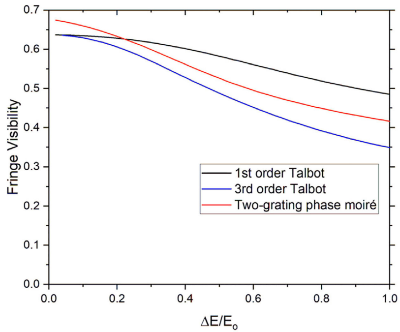
FIGURE 2. Numerical comparison of fringe visibilities of 1st order Talbot interferometer (black), 3rd order Talbot interferometer (blue) and a two-grating phase moiré interferometer (red) under polychromatic point source illumination as functions of the source spectral bandwidth.
