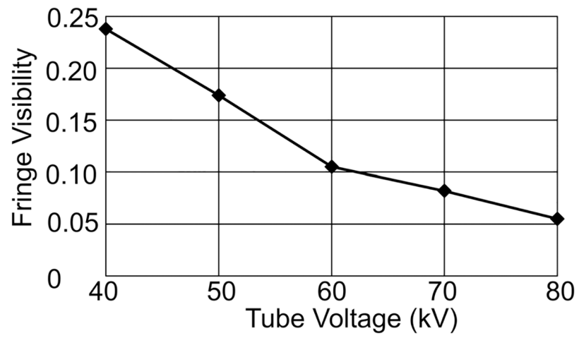
FIGURE 4. The fringe visibility versus tube voltage curve of the four-grating interferometer. Insufficiently thick Au/Si absorption gratings and insufficient phase shift through the moiré phase gratings are responsible for the decrease with x-ray tube voltage.
