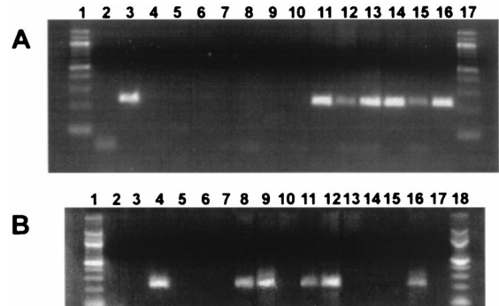
FIG. 7. Detection of BHV-1 DNA in lymphoid tissue and lymphocytes after infection. (A) Pharyngeal tonsil, cervical, retropharyngeal, parotid, and inguinal lymph nodes and trigeminal ganglia were collected from euthanized calves. DNA extraction and PCR conditions were as described in Materials and Methods. Lanes: 1 and 17, molecular weight marker (100-bp DNA ladder); 2, no-template control; 3, MDBK cells infected with BHV-1 for 16 h; 4, mock infected MDBK cells; 5 to 10, pharyngeal tonsil, cervical, retropharyngeal, parotid, and inguinal lymph nodes and trigeminal ganglia, respectively, from a mock-infected calf; 11 to 16, pharyngeal tonsil, cervical, retropharyngeal, parotid, and inguinal lymph nodes and trigeminal ganglia, respectively, from a BHV-1-infected calf (7 dpi). The results are representative of four different infected calves. (B) PBMC were prepared by equilibrium centrifugation. CD4 + and CD8 + lymphocytes were prepared from PBMC and pharyngeal tonsil as described in Materials and Methods. DNA extraction and PCR conditions were as described in Materials and Methods. Lanes: 1 and 18, molecular weight marker (100-bp DNA ladder); 2, no-template control; 3, mock-infected MDBK cells; 4, MDBK cells infected with BHV-1 for 16 h; 5, PBMC from a mock-infected calf; 6 and 7, CD4 + (lane 6) and CD8 + T cells (lane 7) prepared from peripheral blood of a mock-infected calf; 8 to 10, PBMC, CD4 + , and CD8 + cells (peripheral blood), respectively, from a BHV-1-infected calf (5 dpi); 11 to 13, PBMC, CD4 + , and CD8 + cells (peripheral blood), respectively, from a BHV-1-infected calf (7 dpi); 14 and 15, CD4 + (lane 14) and CD8 + (lane 15) cells (pharyngeal tonsil) from a mock-infected calf; 16 and 17, CD4 + (lane 16) and CD8 + (lane 17) cells (pharyngeal tonsil) from a BHV-1-infected calf (7 dpi). Two micrograms of DNA was used for each PCR. The results are representative of four different infected calves.
