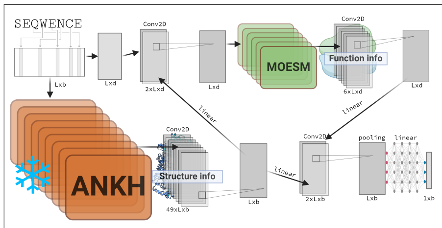
Fig. 3. Model schematic for MOESM8. Frozen ANKH was used to build foundational numerical representations of inputs that a small MOESM added to and modified to be functionally and clustered by EC and GO. The final output was pooled and projected to a single vector for embedding large repositories. Token embedding was modified from explosion.ai. Convolution layers were made with NN-svg. Created with biorender.
