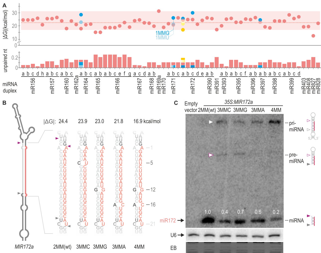
Figure 2. Quantitative regulation of MIRNA processing efficiency by the miRNA/miRNA* secondary structure. (A) Dot plot representing the \Delta G of 62 miRNA duplexes from two-step MIRNA s shown as red dots. A dotted red line shows the mean \Delta G . A red box encloses 95% of the duplexes which have an interacting energy between \sim 17 and 31 kcal/mol. Unpaired nt frequency is shown as red bars on the bottom panel. Blue and yellow dots and bars indicate modifications in the \Delta G and unpaired nt frequency of miRNAs duplex from Figures 1 and 2B, respectively. (B) Schematic representation of MIR172a , the sequence of the wt and mutant miRNA duplexes is shown to the right. These depictions are based on mfold secondary structure prediction (see Appendix II). Black letters specify the introduced mismatches, and the numbers indicate their position counting from the 5' end of the miRNA. MiRNA is shown in red and miRNA* in grey. \Delta G of the duplex are shown above each small RNA sequence. (C) Small RNA blot for miR172 transgenic lines expressing different precursors from the 35S promoter. Each sample corresponds to 15 pooled 10-day-old seedlings from independent primary transgenic plants. Numbers above small RNA blots correspond to miRNA levels quantified relative to the wt precursor. Schematic representation of the detected MIR172 processing intermediates is shown on the right. A grey empty arrow and purple empty arrow indicate the pri-miRNA and pre-miRNA detected in the blot, respectively. Both U6 hybridization and EB staining are shown at the bottom.
