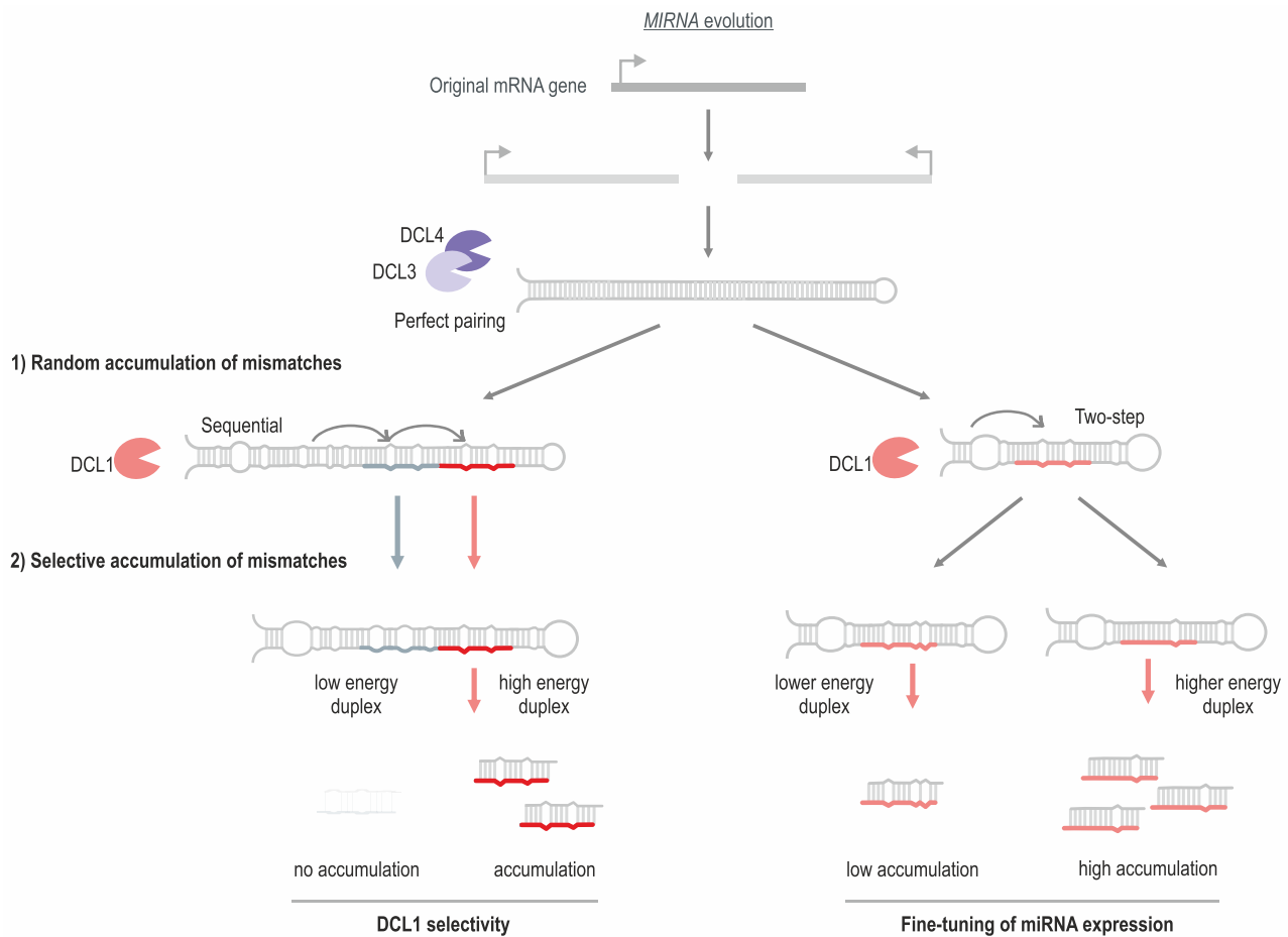
Figure 7. Proposed model of MIRNA evolution. A protein-coding gene undergoes an inverted duplication, generating a hairpin that is processed by DCL3 and/or DCL4. The processing of this proto- MIRNA generates a diverse mixture of small RNAs. In the next stage, the accumulation of mutations determines that the fold-back is processed by DCL1 and establishes the structural determinants for its first cut. In a subsequent stage, mutations in the small RNA duplex region of the precursor provide specificity for selected miRNAs in sequential MIRNA s, while mutations in the two-step precursors determine the quantitative levels of miRNA biogenesis.
