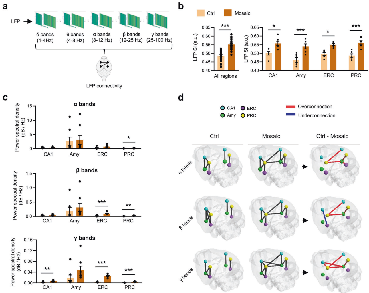
Fig. 6 Pcdh19 mosaic mice show hyperconnectivity among limbic system areas. a Experimental workflow scheme: extracellular neuronal activity was analyzed to obtain LFP signals at discrete frequency bands (1–100 Hz interval) and extrapolate functional connectivity between limbic system areas. b LFP SI relative to recordings in all limbic system regions (left) and in single regions (right) from mosaic mice ( Pcdh19 fl/y Syn1-Cre, Mosaic ) and controls ( Pcdh19 fl/y , Ctrl ) (N, 5-7 recording sessions/brain region/mouse, 2 mice/genotype; Student's t -test, * p < 0.05, *** p < 0.001). c LFP power spectral density in α, β, and γ bands from limbic system regions of mice as in b (N, 5-7 recording sessions/brain region/mouse, 2 mice/genotype; Student's t -test, * p < 0.05, ** p < 0.01, *** p < 0.001). d Connectome maps illustrating functional connections between limbic system regions of the ipsi- and contralateral hemisphere, extrapolated from LFP signals in α, β and γ bands in mice as in b . Differential connections emerging from the comparison between the two groups are shown in red (overconnections in Mosaic mice) and blue (underconnections in Mosaic mice). All data ( b , c ) are shown as means ± SEM. See also Supplementary Table 6.
