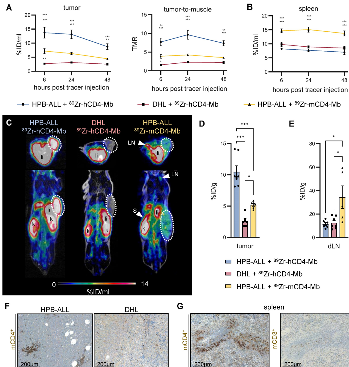
Figure 2. In vivo ^{89}\text{Zr-hCD4-Mb} and ^{89}\text{Zr-mCD4-Mb} binding to \text{CD4}^+ cells in immunodeficient NSG mice. (A) In vivo PET uptake quantification and tumor-to-muscle ratio of \text{hCD4}^+ HPB-ALL and \text{hCD4}^+ DHL xenografts 6, 24, and 48 h after ^{89}\text{Zr-hCD4-Mb} or ^{89}\text{Zr-mCD4-Mb} injection. (B) In vivo PET uptake quantification of the spleen. (C) Representative PET/MR images acquired 48 h after ^{89}\text{Zr-hCD4-Mb} or ^{89}\text{Zr-mCD4-Mb} injection. Tumors are highlighted with a white circle. LN: lymph nodes; s: spleen; k: kidney; li: liver. (D) Ex vivo biodistribution of \text{hCD4}^+ HPB-ALL and \text{hCD4}^+ DHL tumors and (E) draining lymph nodes (dLNs) measured by \gamma -counting at 48 h after ^{89}\text{Zr-hCD4-Mb} or ^{89}\text{Zr-mCD4-Mb} injection. (F) Ex vivo immunohistochemistry (IHC) of endogenous \text{mCD4}^+ cells from HPB-ALL tumors and DHL tumors of NSG mice. (G) Ex vivo IHC of endogenous \text{mCD4}^+ cells and \text{mCD3}^+ cells from the spleens of NSG mice. P values were calculated by two-way ANOVA (A, B) or ordinary one-way ANOVA (D, E) using the Tukey post-hoc test. Data derived from two independent experiments ( n = 6-7 per group). * p < 0.05 , ** p < 0.01 , *** p < 0.001 .
