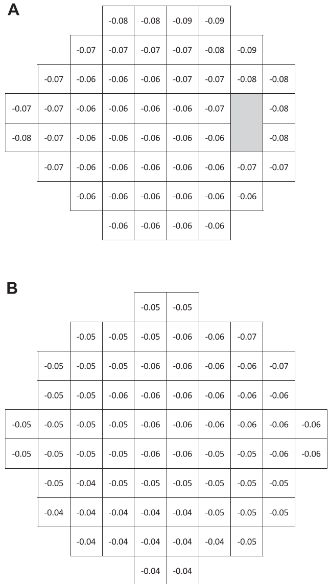
Figure 2. Pointwise cross-sectional age rate of decline in average sensitivity across the tested 24-degree (A) and 10-degree (B) fields of TEMPO.
