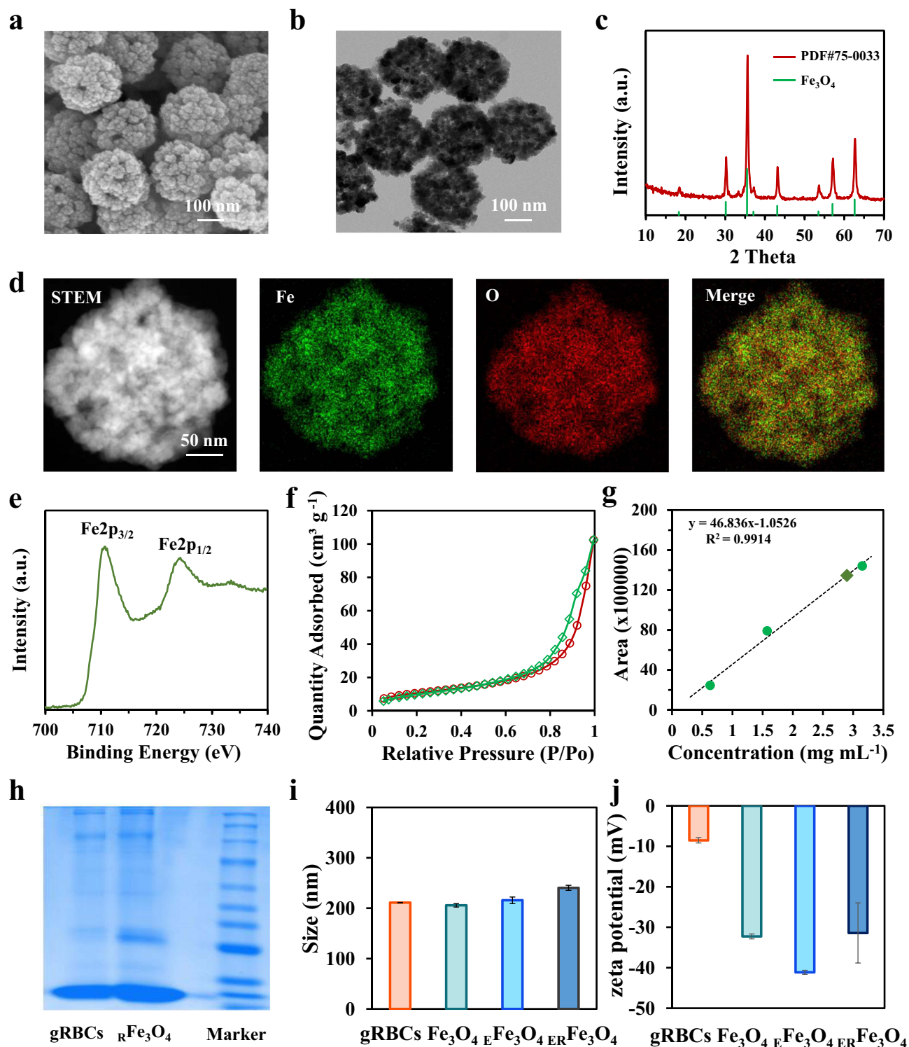
Figure 2 Physicochemical characterization of \text{ERFe}_3\text{O}_4 NPs. (a) SEM image and (b) TEM image of hollow \text{Fe}_3\text{O}_4 NPs. (c) XRD pattern, (d) STEM and the elemental mapping images of hollow \text{Fe}_3\text{O}_4 NPs. (e) XPS spectra of Fe2p region of hollow \text{Fe}_3\text{O}_4 NPs. (f) \text{N}_2 adsorption/desorption isotherm of hollow \text{Fe}_3\text{O}_4 NPs. (g) A calibration curve using HPLC spectroscopy was employed to assess the efficiency of emodin loading. (h) Protein analysis of gRBCs, \text{rFe}_3\text{O}_4 NPs and Marker by using SDS-PAGE. Samples were stained with Coomassie Brilliant. (i) Size and (j) Zeta potential of gRBCs, \text{Fe}_3\text{O}_4 NPs, \text{eFe}_3\text{O}_4 NPs and \text{ERFe}_3\text{O}_4 NPs.
