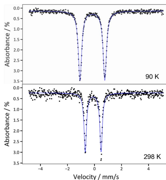
Fig. 3 Zero-field ^{57}\text{Fe} Mössbauer spectra of 2 collected at T = 90 \text{ K} (top) and T = 298 \text{ K} (bottom). The blue traces correspond to the overall fits, which are described in the main text.
