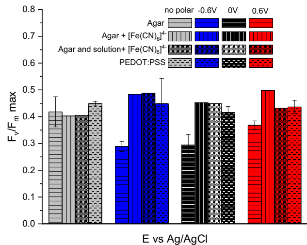
Fig. 8 Maximum photoconversion yields for cyanobacteria embedded in mediator-free agar in PBS solution, agar with [\text{Fe}(\text{CN})_6]^{4-} in PBS solution and agar with [\text{Fe}(\text{CN})_6]^{4-} in [\text{Fe}(\text{CN})_6]^{4-} containing PBS solution, and in PEDOT:PSS.
