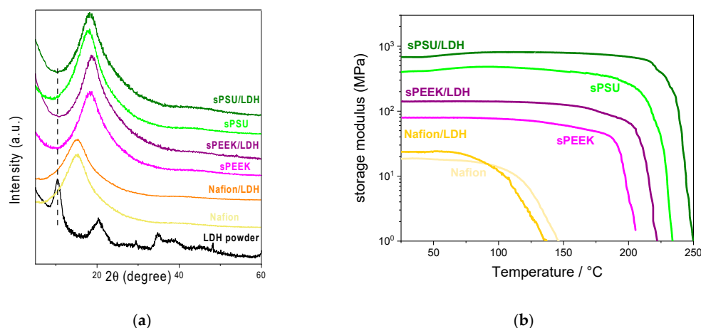
Figure 3. (a) XRD patterns and (b) DMA thermograms for the Nafion-based, sPEEK-based, and sPSU-based membranes.
